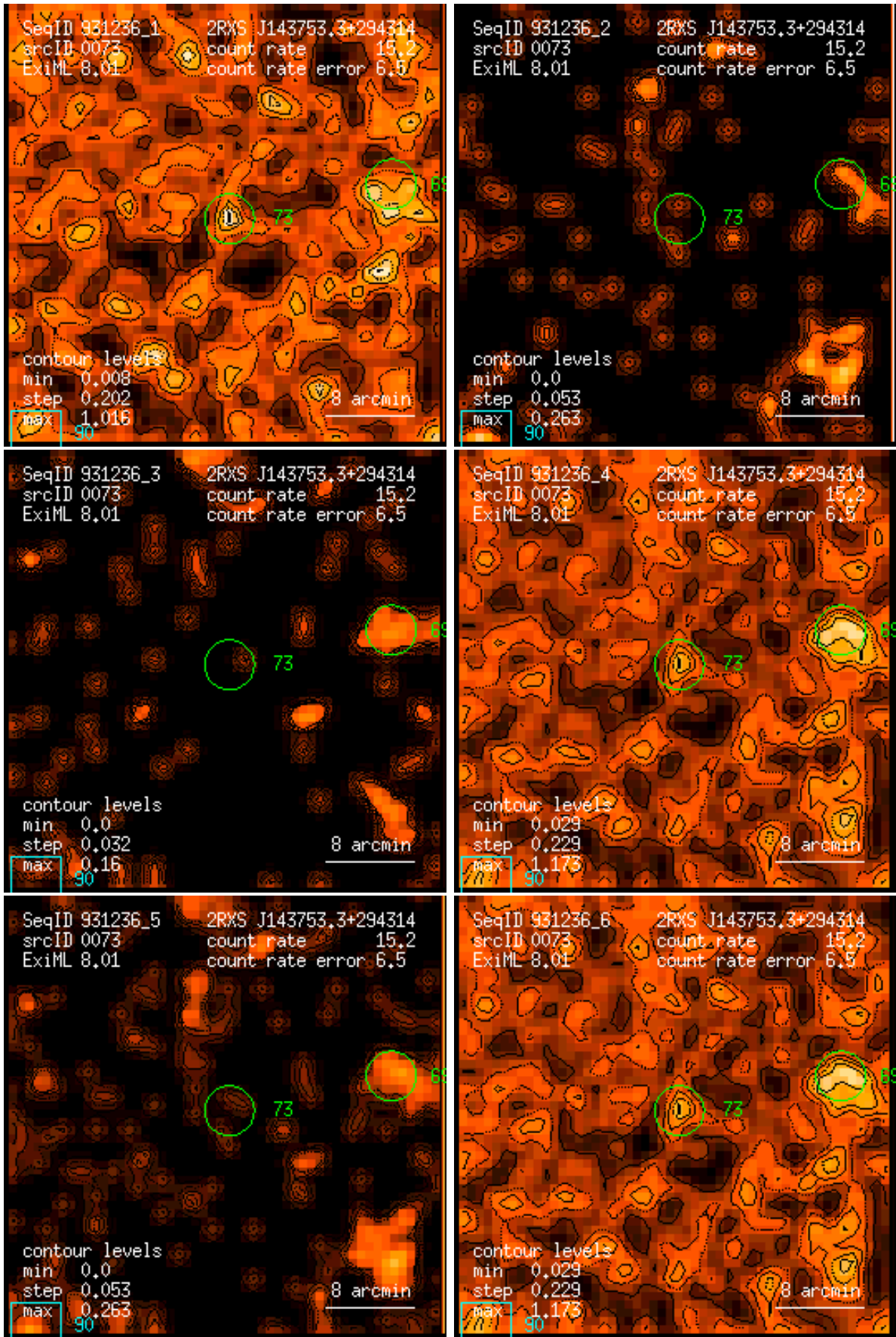
Figure 73: RASS 931236: detection 0073: band rate images, Gaussian filter: (1) PSPC channels 11 – 41, (2) 52 – 90, (3) 91 – 201, (4) 11 – 235, (5) 52 – 201, (6) 11 – 201. Broad band rates in counts/ks. Band rate contour levels in counts/ks/arcmin 2 .
