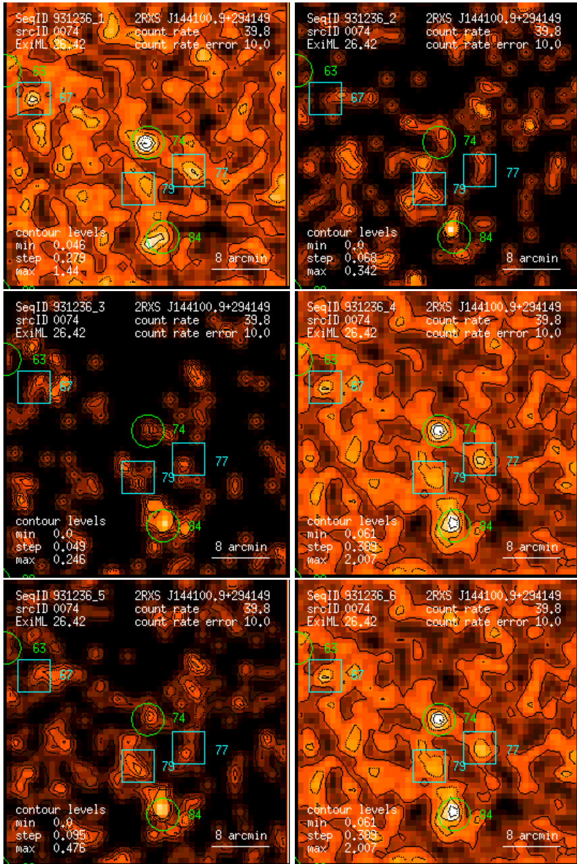
Figure 74: RASS 931236: detection 0074: band rate images, Gaussian filter: (1) PSPC channels 11 – 41, (2) 52 – 90, (3) 91 – 201, (4) 11 – 235, (5) 52 – 201, (6) 11 – 201. Broad band rates in counts/ks. Band rate contour levels in counts/ks/arcmin 2 .
