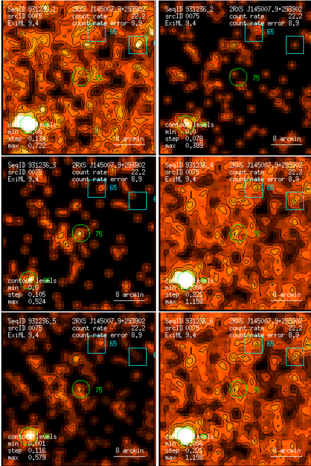
Figure 75: RASS 931236: detection 0075: band rate images, Gaussian filter: (1) PSPC channels 11 – 41, (2) 52 – 90, (3) 91 – 201, (4) 11 – 235, (5) 52 – 201, (6) 11 – 201. Broad band rates in counts/ks. Band rate contour levels in counts/ks/arcmin 2 .
