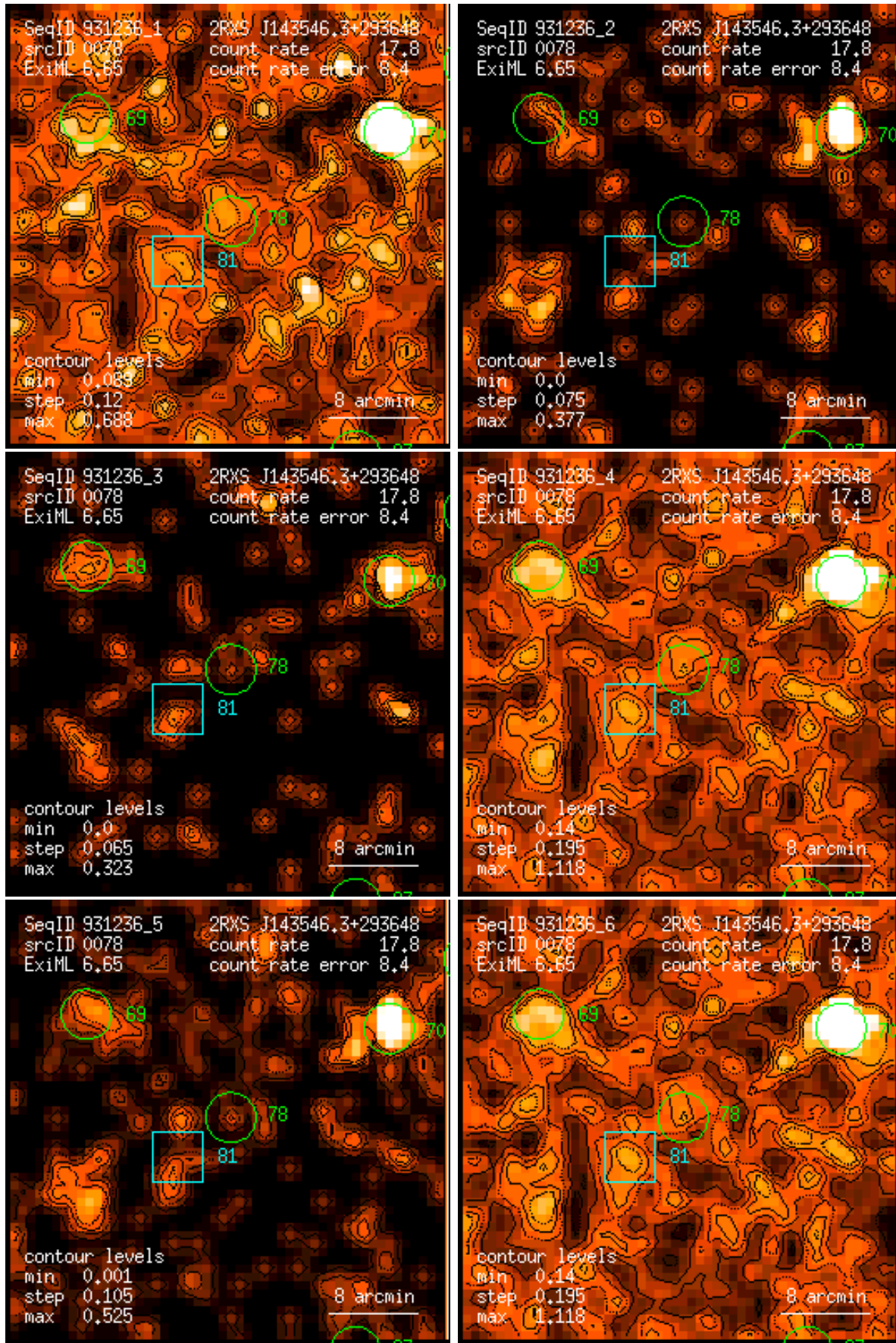
Figure 78: RASS 931236: detection 0078: band rate images, Gaussian filter: (1) PSPC channels 11 – 41, (2) 52 – 90, (3) 91 – 201, (4) 11 – 235, (5) 52 – 201, (6) 11 – 201. Broad band rates in counts/ks. Band rate contour levels in counts/ks/arcmin 2 .
