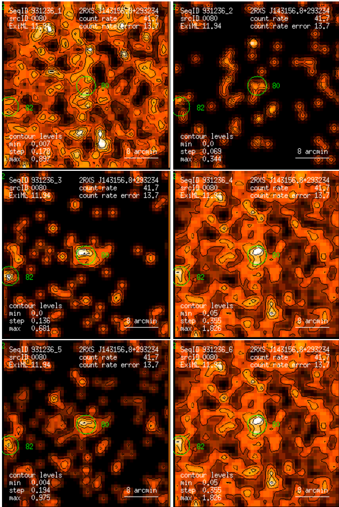
Figure 80: RASS 931236: detection 0080: band rate images, Gaussian filter: (1) PSPC channels 11 – 41, (2) 52 – 90, (3) 91 – 201, (4) 11 – 235, (5) 52 – 201, (6) 11 – 201. Broad band rates in counts/ks. Band rate contour levels in counts/ks/arcmin 2 .
