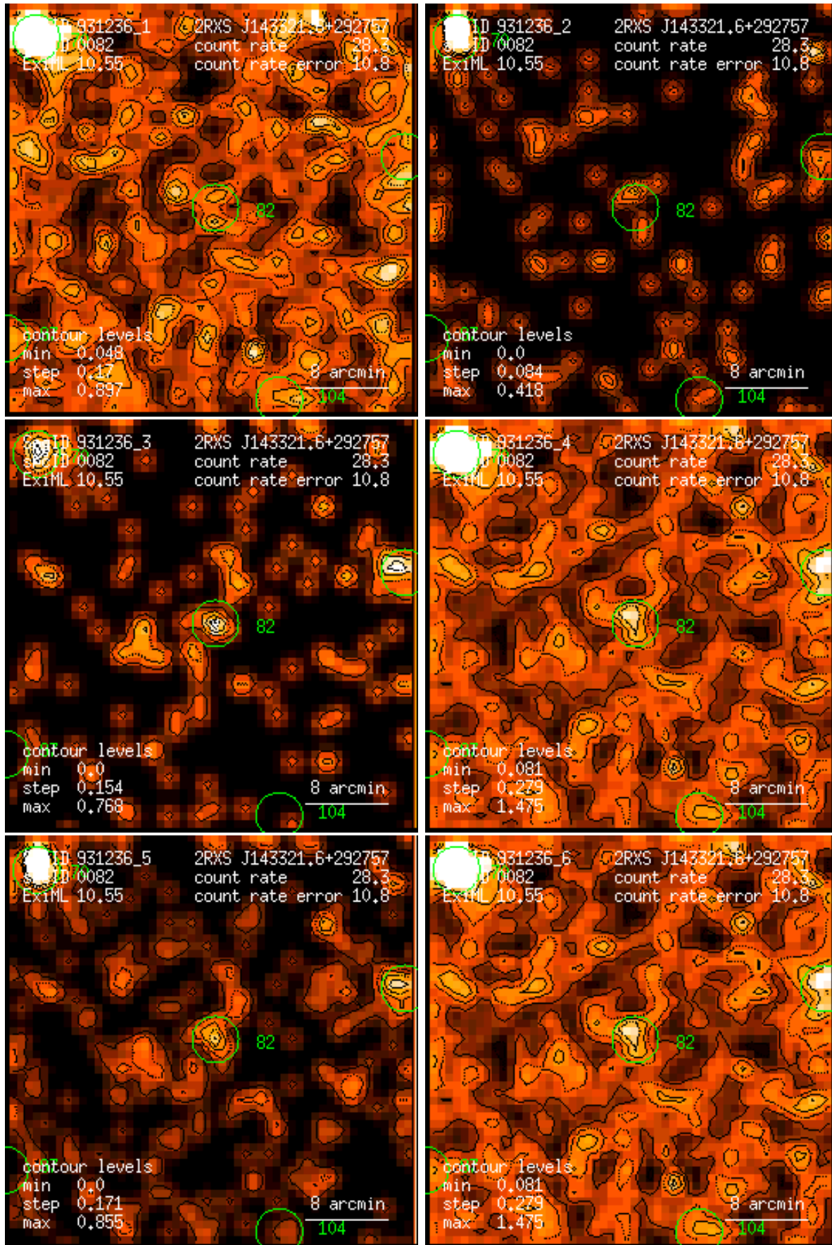
Figure 82: RASS 931236: detection 0082: band rate images, Gaussian filter: (1) PSPC channels 11 – 41, (2) 52 – 90, (3) 91 – 201, (4) 11 – 235, (5) 52 – 201, (6) 11 – 201. Broad band rates in counts/ks. Band rate contour levels in counts/ks/arcmin 2 .
