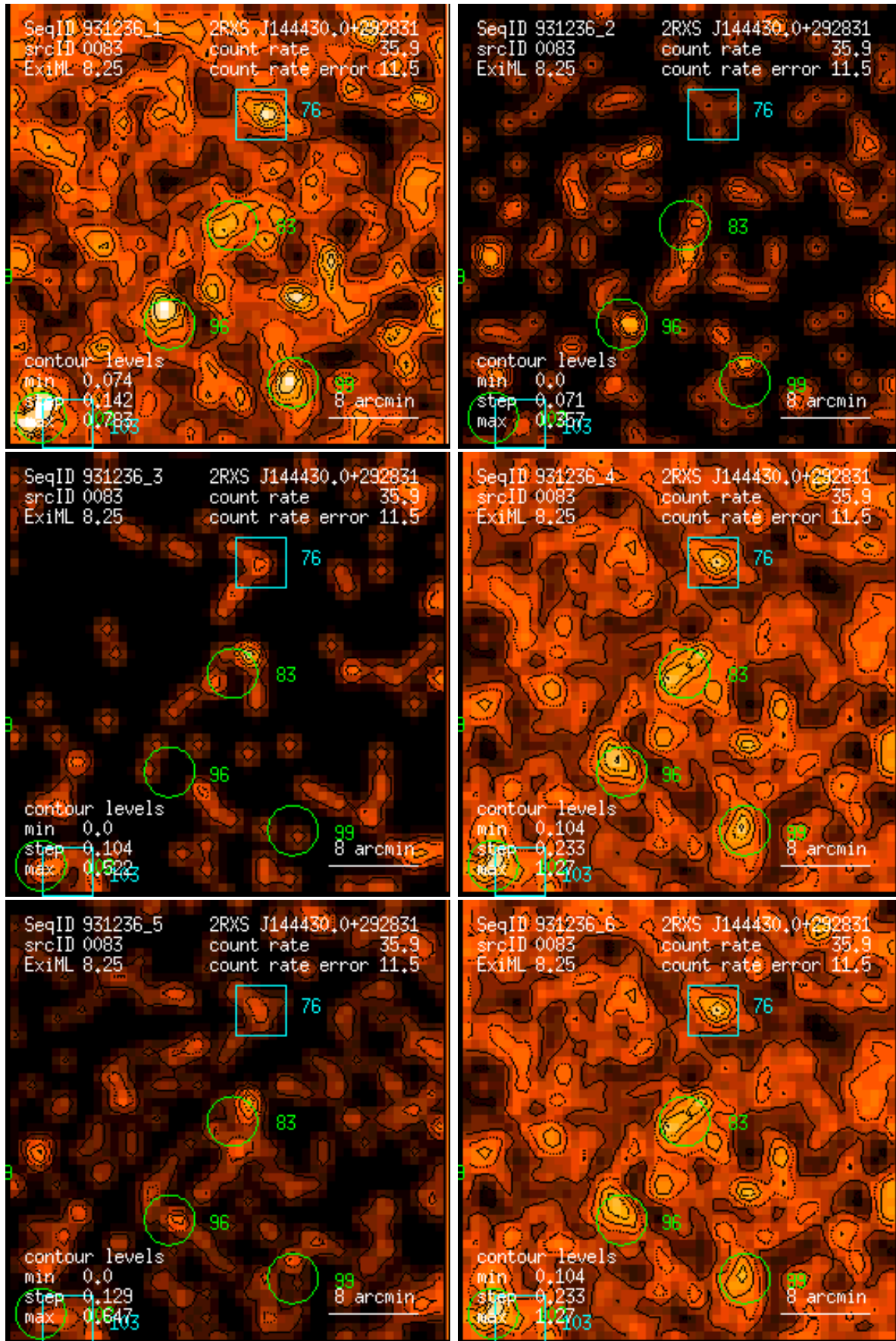
Figure 83: RASS 931236: detection 0083: band rate images, Gaussian filter: (1) PSPC channels 11 – 41, (2) 52 – 90, (3) 91 – 201, (4) 11 – 235, (5) 52 – 201, (6) 11 – 201. Broad band rates in counts/ks. Band rate contour levels in counts/ks/arcmin 2 .
