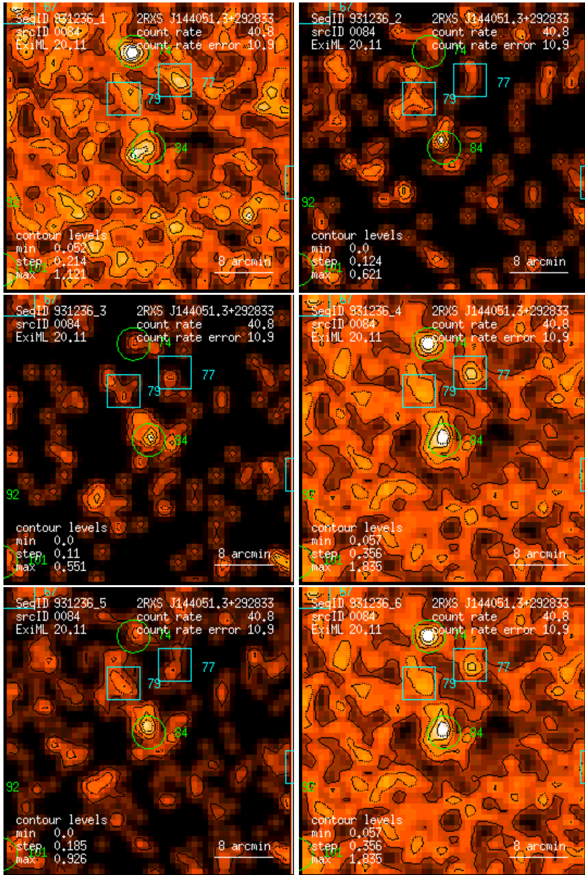
Figure 84: RASS 931236: detection 0084: band rate images, Gaussian filter: (1) PSPC channels 11 – 41, (2) 52 – 90, (3) 91 – 201, (4) 11 – 235, (5) 52 – 201, (6) 11 – 201. Broad band rates in counts/ks. Band rate contour levels in counts/ks/arcmin 2 .
