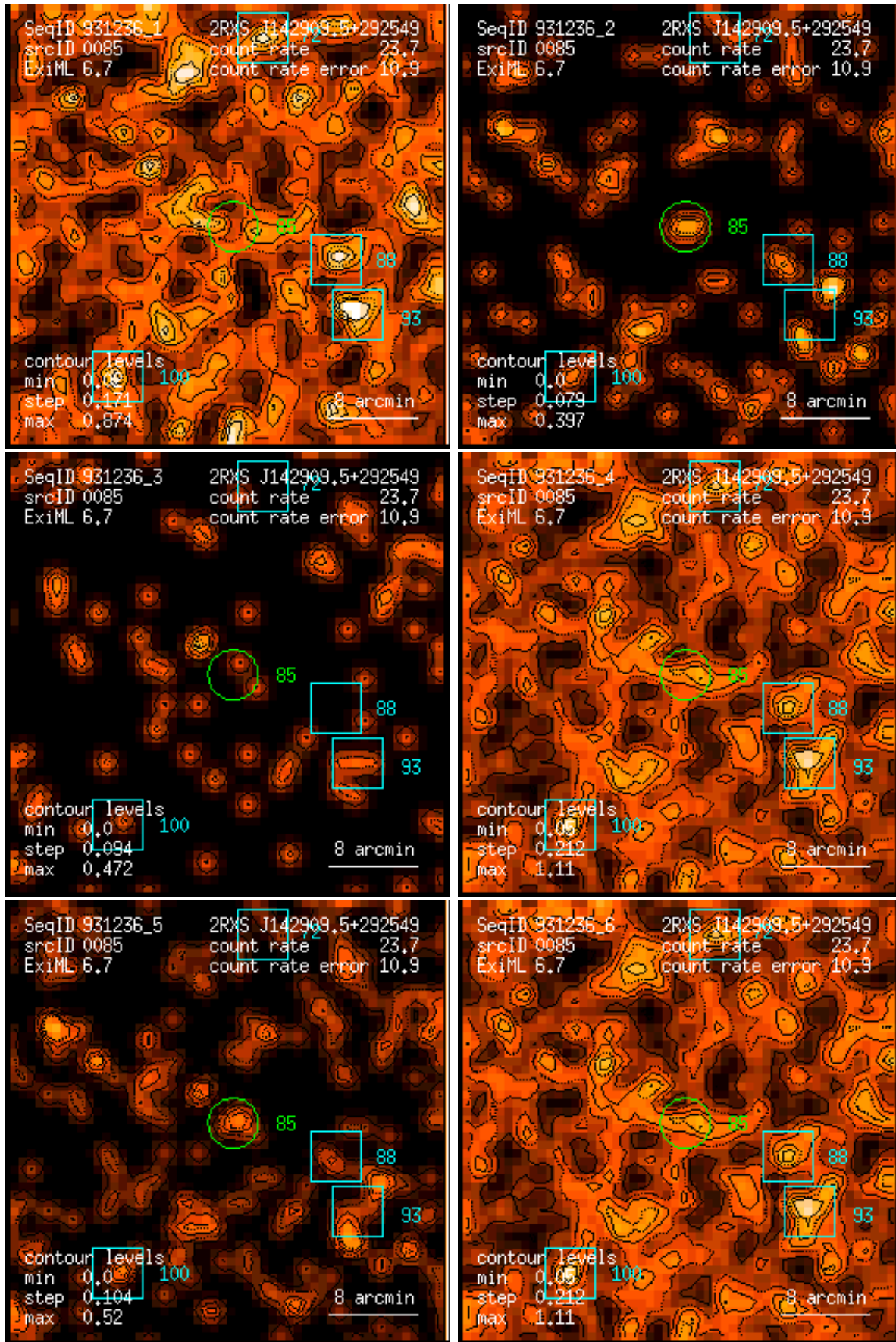
Figure 85: RASS 931236: detection 0085: band rate images, Gaussian filter: (1) PSPC channels 11 – 41, (2) 52 – 90, (3) 91 – 201, (4) 11 – 235, (5) 52 – 201, (6) 11 – 201. Broad band rates in counts/ks. Band rate contour levels in counts/ks/arcmin 2 .
