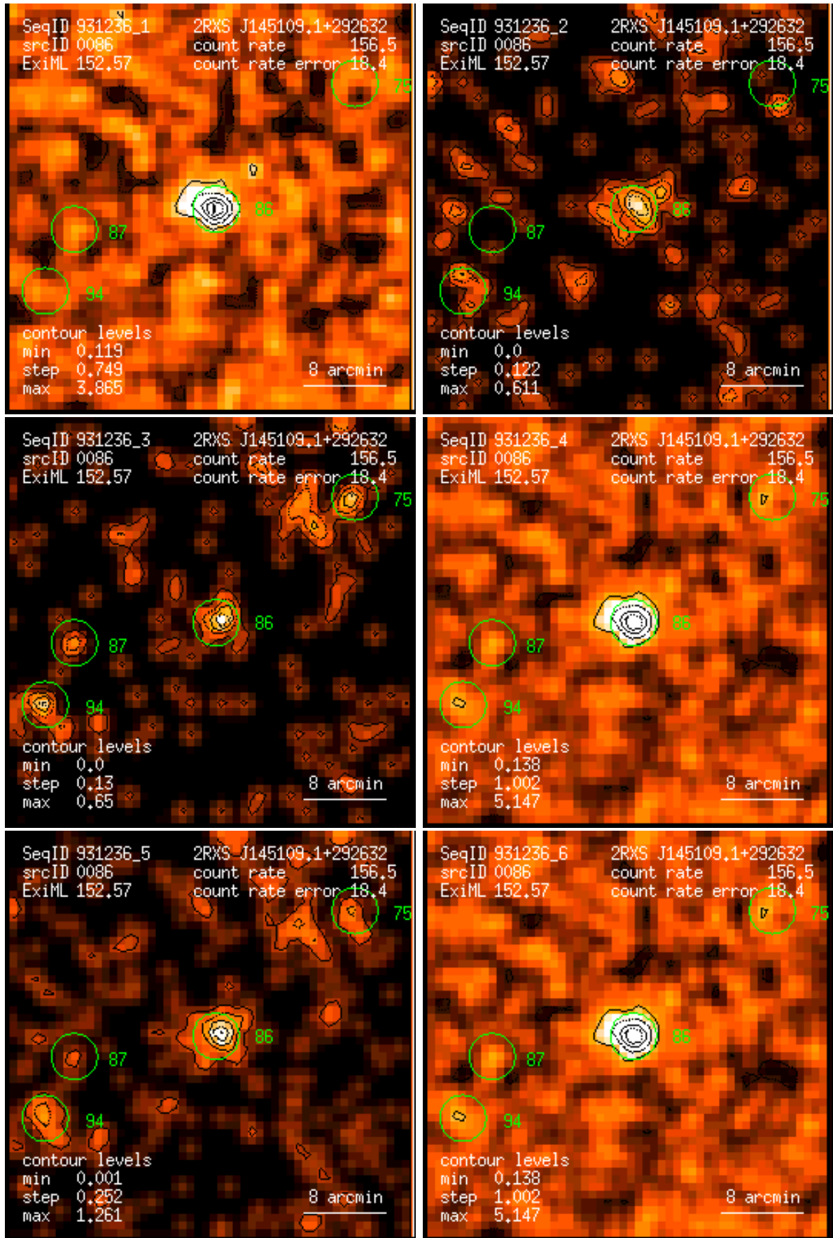
Figure 86: RASS 931236: detection 0086: band rate images, Gaussian filter: (1) PSPC channels 11 – 41, (2) 52 – 90, (3) 91 – 201, (4) 11 – 235, (5) 52 – 201, (6) 11 – 201. Broad band rates in counts/ks. Band rate contour levels in counts/ks/arcmin 2 .
