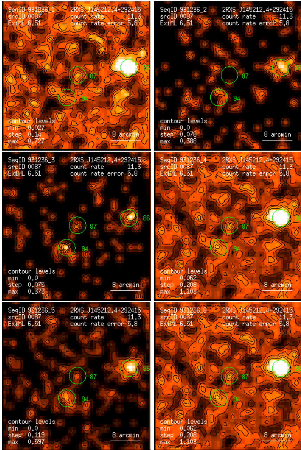
Figure 87: RASS 931236: detection 0087: band rate images, Gaussian filter: (1) PSPC channels 11 – 41, (2) 52 – 90, (3) 91 – 201, (4) 11 – 235, (5) 52 – 201, (6) 11 – 201. Broad band rates in counts/ks. Band rate contour levels in counts/ks/arcmin 2 .
