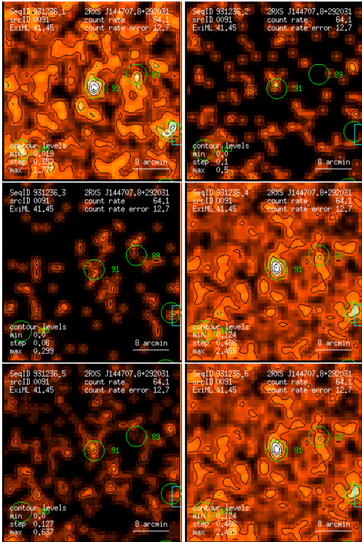
Figure 91: RASS 931236: detection 0091: band rate images, Gaussian filter: (1) PSPC channels 11 – 41, (2) 52 – 90, (3) 91 – 201, (4) 11 – 235, (5) 52 – 201, (6) 11 – 201. Broad band rates in counts/ks. Band rate contour levels in counts/ks/arcmin 2 .
