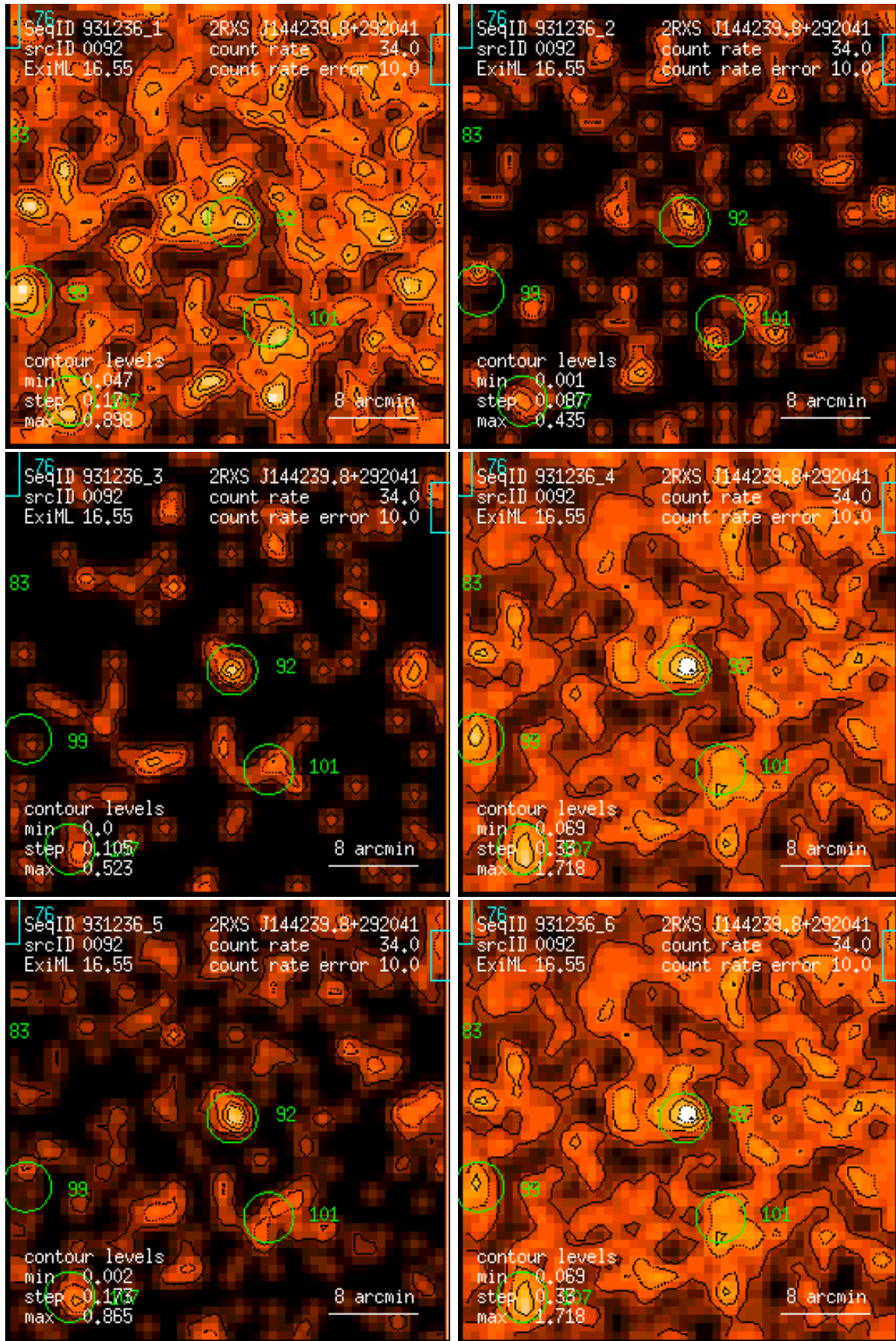
Figure 92: RASS 931236: detection 0092: band rate images, Gaussian filter: (1) PSPC channels 11 – 41, (2) 52 – 90, (3) 91 – 201, (4) 11 – 235, (5) 52 – 201, (6) 11 – 201. Broad band rates in counts/ks. Band rate contour levels in counts/ks/arcmin 2 .
