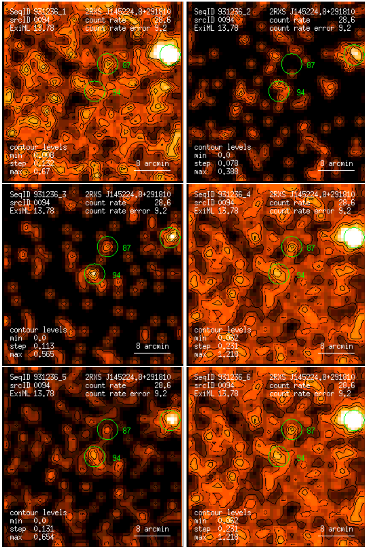
Figure 94: RASS 931236: detection 0094: band rate images, Gaussian filter: (1) PSPC channels 11 – 41, (2) 52 – 90, (3) 91 – 201, (4) 11 – 235, (5) 52 – 201, (6) 11 – 201. Broad band rates in counts/ks. Band rate contour levels in counts/ks/arcmin 2 .
