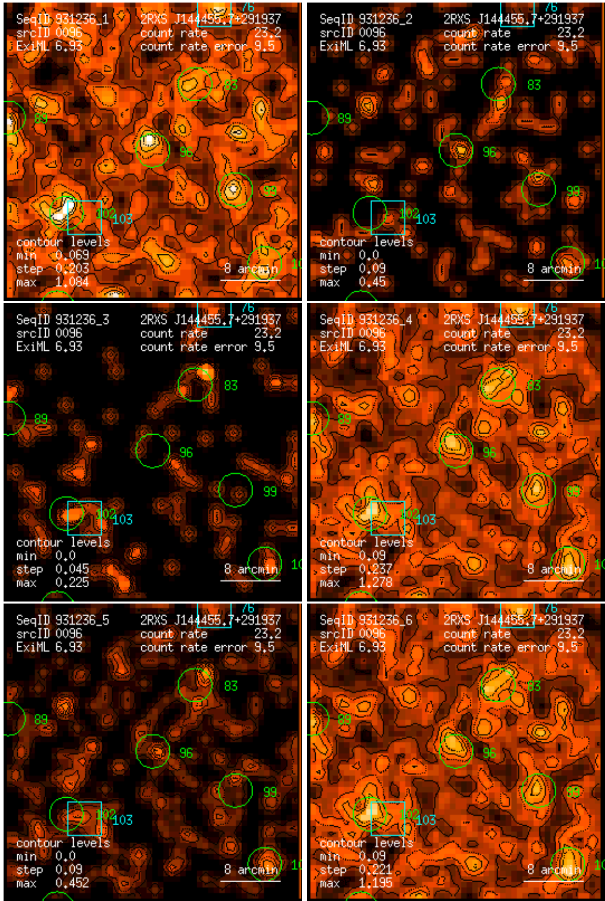
Figure 96: RASS 931236: detection 0096: band rate images, Gaussian filter: (1) PSPC channels 11 – 41, (2) 52 – 90, (3) 91 – 201, (4) 11 – 235, (5) 52 – 201, (6) 11 – 201. Broad band rates in counts/ks. Band rate contour levels in counts/ks/arcmin 2 .
