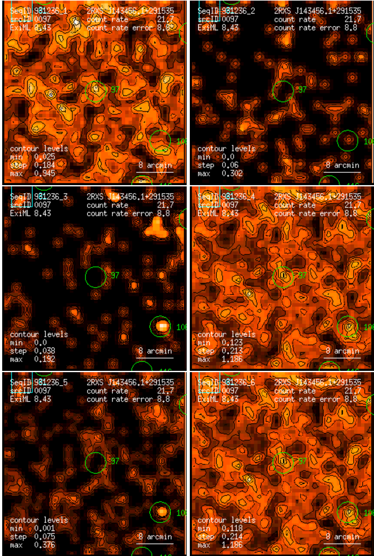
Figure 97: RASS 931236: detection 0097: band rate images, Gaussian filter: (1) PSPC channels 11 – 41, (2) 52 – 90, (3) 91 – 201, (4) 11 – 235, (5) 52 – 201, (6) 11 – 201. Broad band rates in counts/ks. Band rate contour levels in counts/ks/arcmin 2 .
