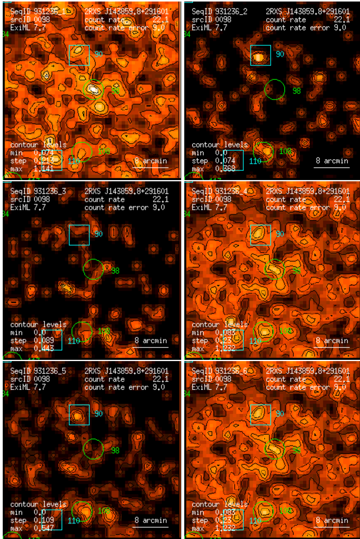
Figure 98: RASS 931236: detection 0098: band rate images, Gaussian filter: (1) PSPC channels 11 – 41, (2) 52 – 90, (3) 91 – 201, (4) 11 – 235, (5) 52 – 201, (6) 11 – 201. Broad band rates in counts/ks. Band rate contour levels in counts/ks/arcmin 2 .
