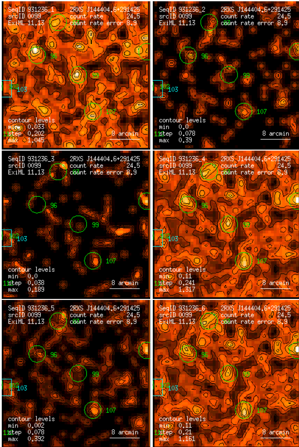
Figure 99: RASS 931236: detection 0099: band rate images, Gaussian filter: (1) PSPC channels 11 – 41, (2) 52 – 90, (3) 91 – 201, (4) 11 – 235, (5) 52 – 201, (6) 11 – 201. Broad band rates in counts/ks. Band rate contour levels in counts/ks/arcmin 2 .
