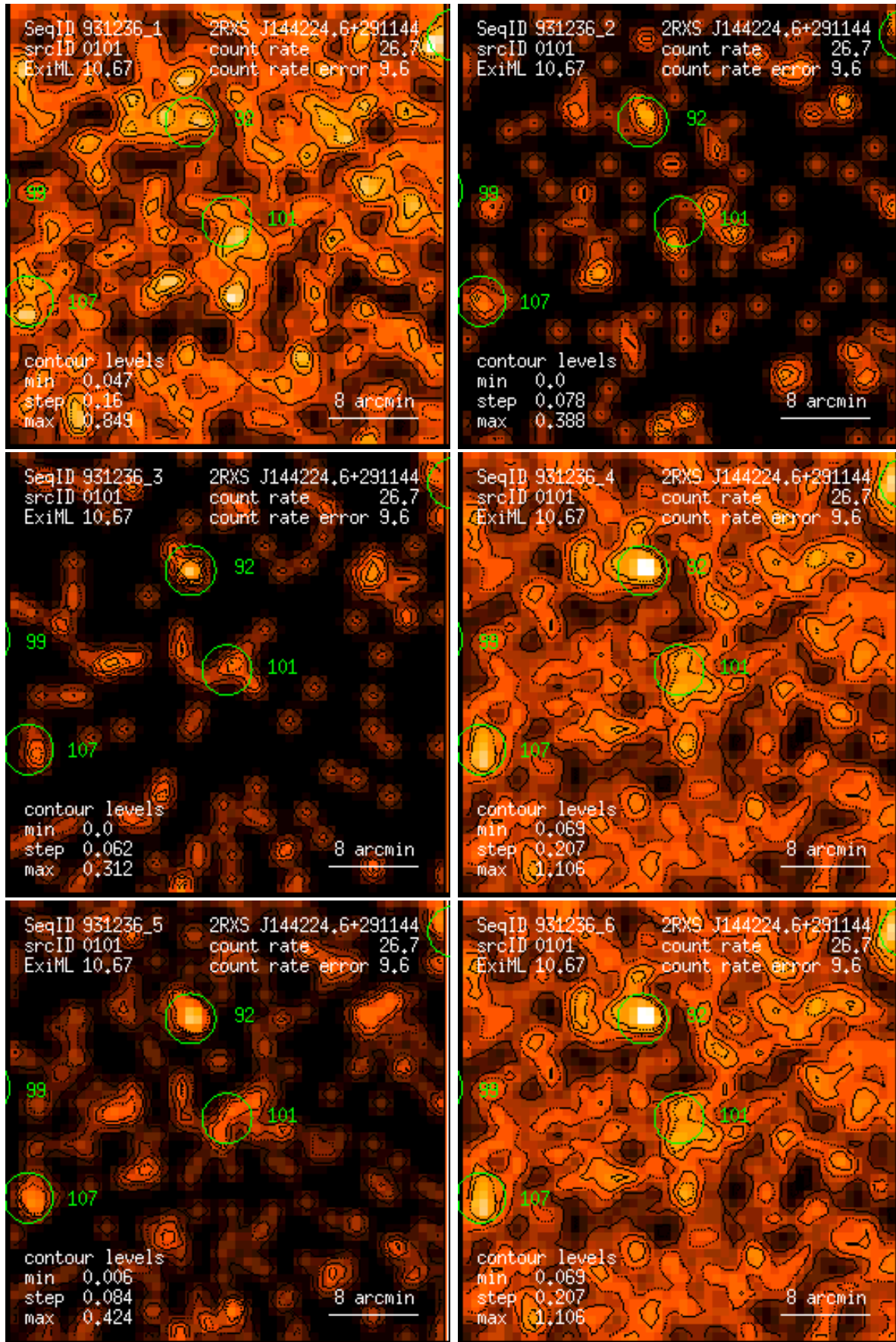
Figure 101: RASS 931236: detection 0101: band rate images, Gaussian filter: (1) PSPC channels 11 – 41, (2) 52 – 90, (3) 91 – 201, (4) 11 – 235, (5) 52 – 201, (6) 11 – 201. Broad band rates in counts/ks. Band rate contour levels in counts/ks/arcmin 2 .
