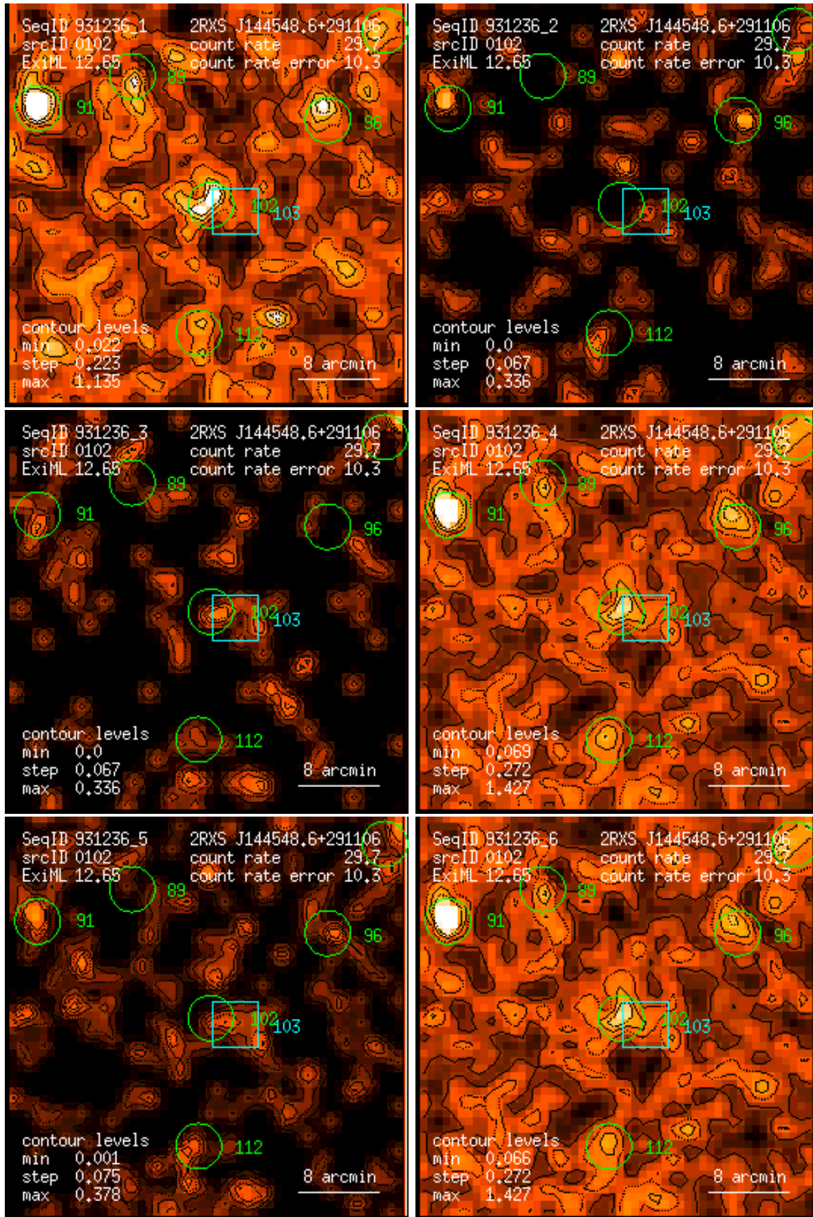
Figure 102: RASS 931236: detection 0102: band rate images, Gaussian filter: (1) PSPC channels 11 – 41, (2) 52 – 90, (3) 91 – 201, (4) 11 – 235, (5) 52 – 201, (6) 11 – 201. Broad band rates in counts/ks. Band rate contour levels in counts/ks/arcmin 2 .
