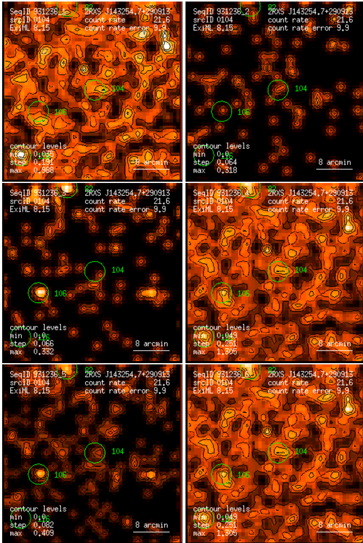
Figure 104: RASS 931236: detection 0104: band rate images, Gaussian filter: (1) PSPC channels 11 – 41, (2) 52 – 90, (3) 91 – 201, (4) 11 – 235, (5) 52 – 201, (6) 11 – 201. Broad band rates in counts/ks. Band rate contour levels in counts/ks/arcmin 2 .
