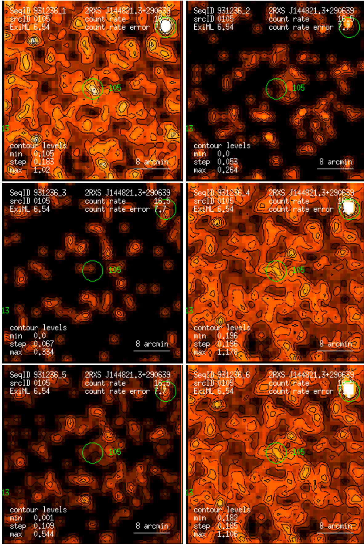
Figure 105: RASS 931236: detection 0105: band rate images, Gaussian filter: (1) PSPC channels 11 – 41, (2) 52 – 90, (3) 91 – 201, (4) 11 – 235, (5) 52 – 201, (6) 11 – 201. Broad band rates in counts/ks. Band rate contour levels in counts/ks/arcmin 2 .
