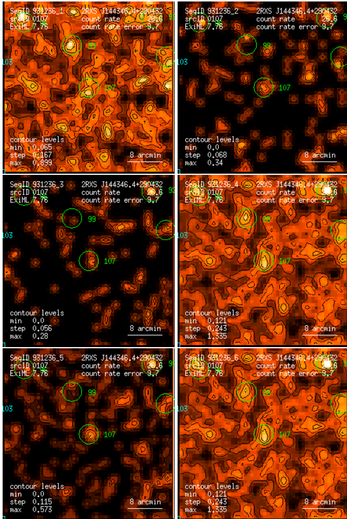
Figure 107: RASS 931236: detection 0107: band rate images, Gaussian filter: (1) PSPC channels 11 – 41, (2) 52 – 90, (3) 91 – 201, (4) 11 – 235, (5) 52 – 201, (6) 11 – 201. Broad band rates in counts/ks. Band rate contour levels in counts/ks/arcmin 2 .
