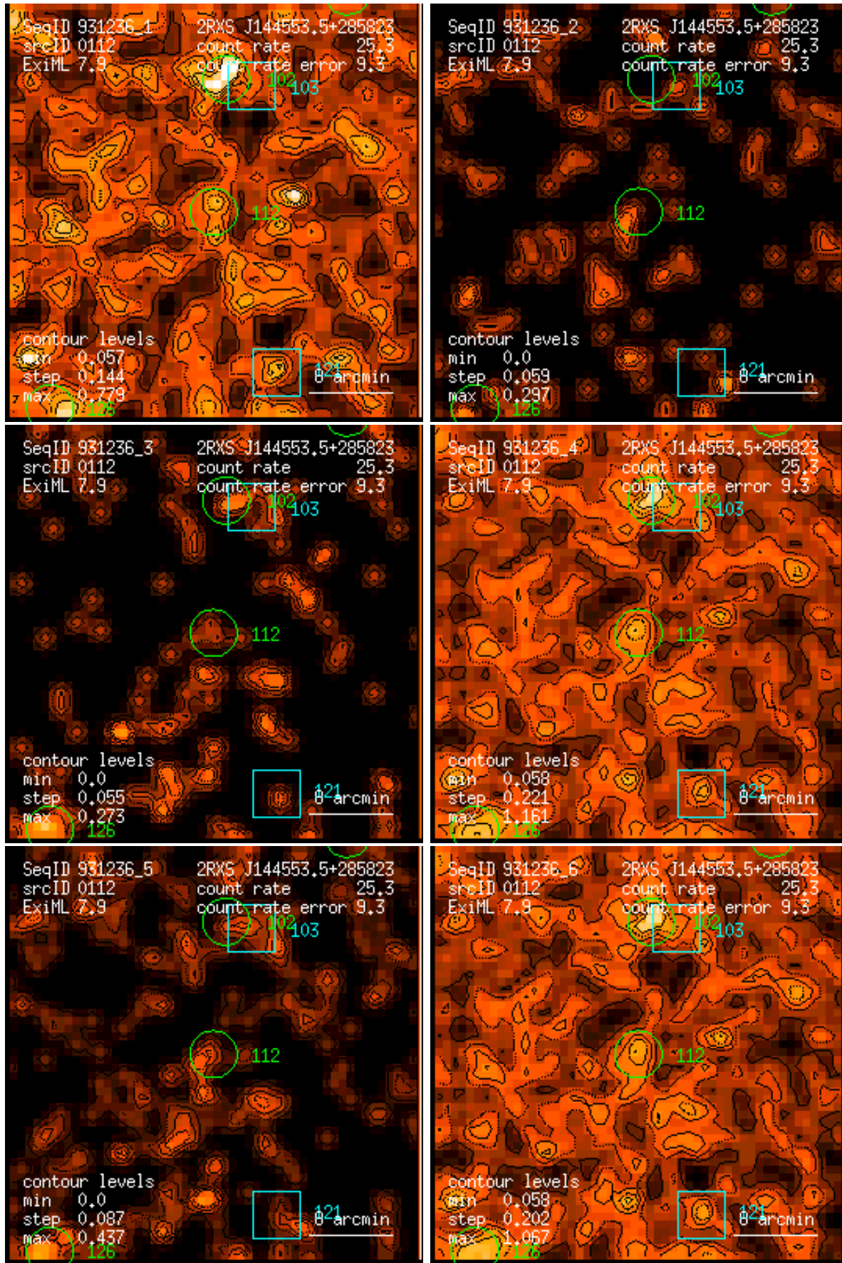
Figure 112: RASS 931236: detection 0112: band rate images, Gaussian filter: (1) PSPC channels 11 – 41, (2) 52 – 90, (3) 91 – 201, (4) 11 – 235, (5) 52 – 201, (6) 11 – 201. Broad band rates in counts/ks. Band rate contour levels in counts/ks/arcmin 2 .
