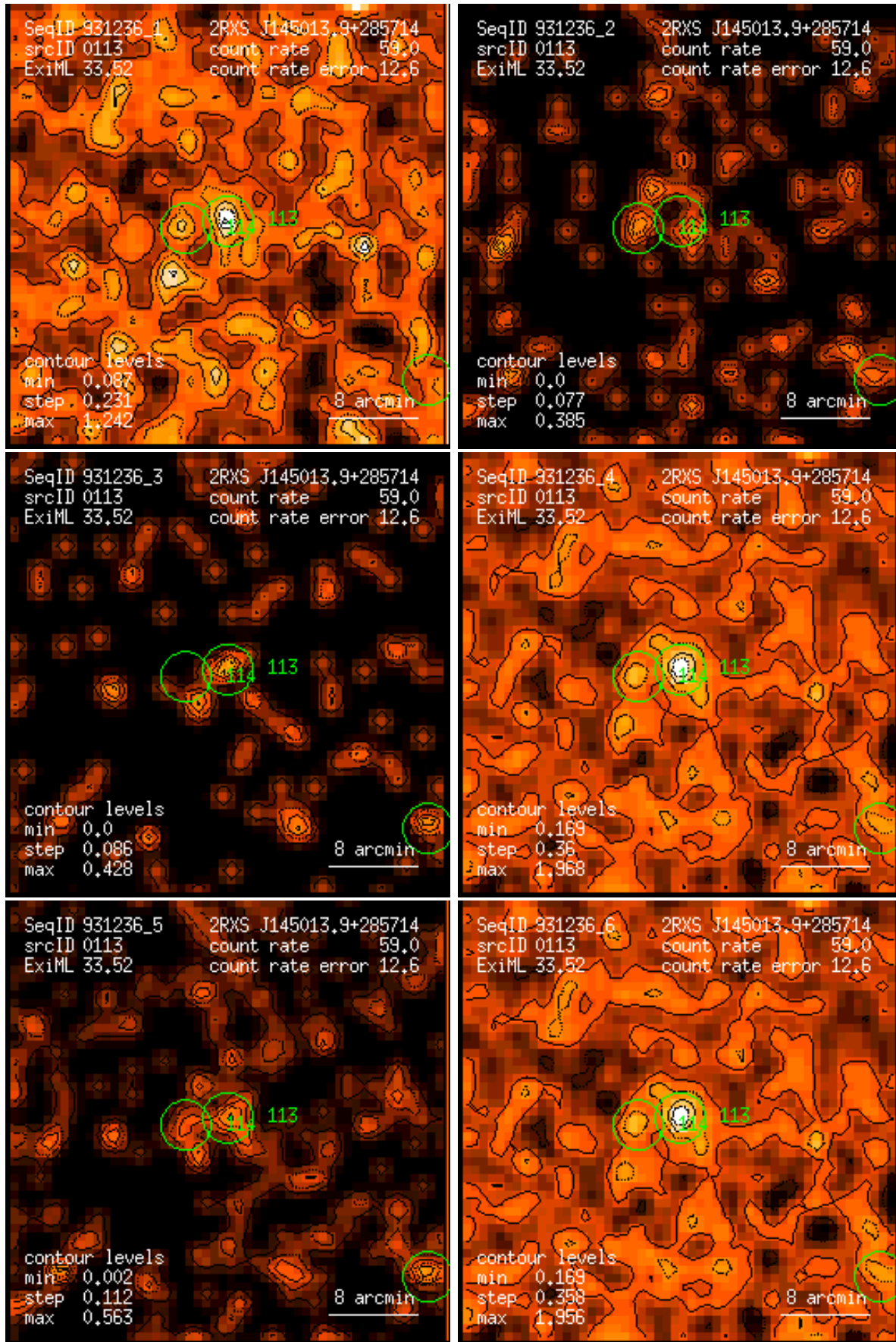
Figure 113: RASS 931236: detection 0113: band rate images, Gaussian filter: (1) PSPC channels 11 – 41, (2) 52 – 90, (3) 91 – 201, (4) 11 – 235, (5) 52 – 201, (6) 11 – 201. Broad band rates in counts/ks. Band rate contour levels in counts/ks/arcmin 2 .
