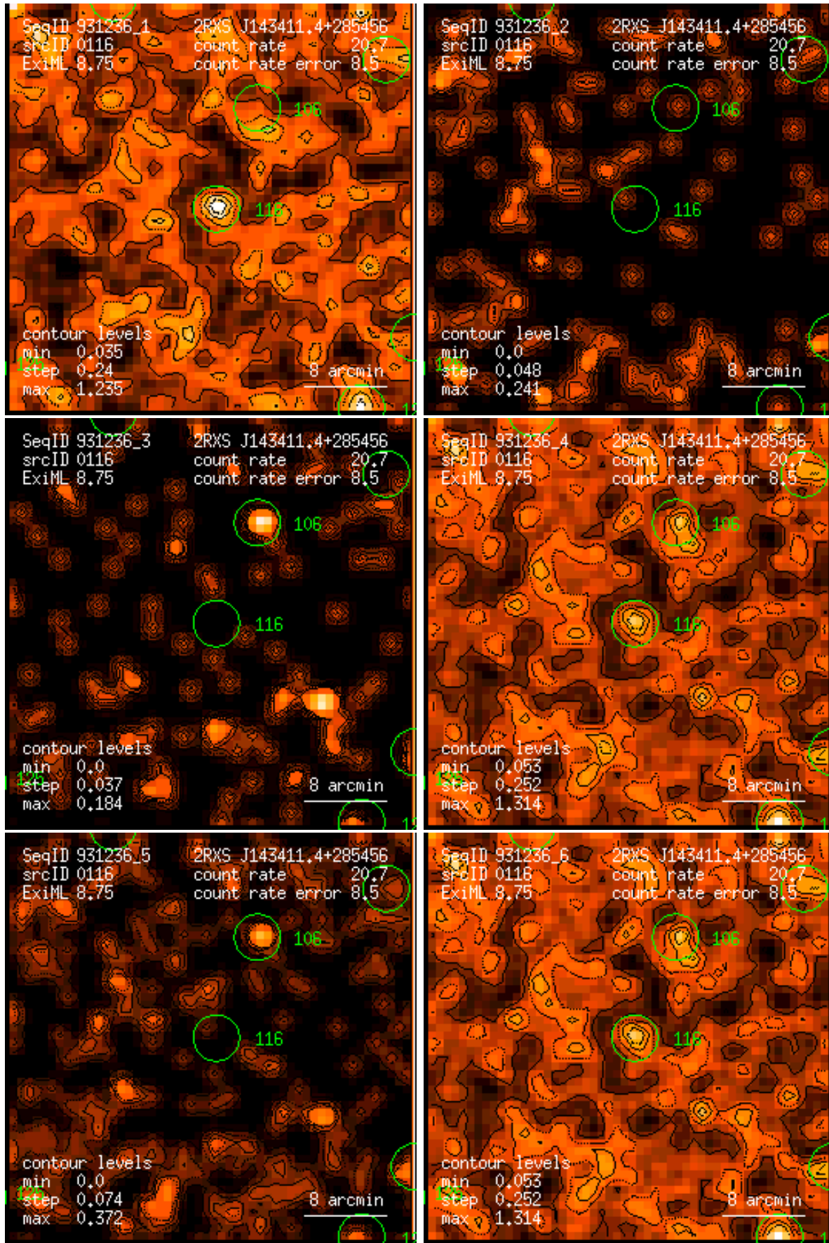
Figure 116: RASS 931236: detection 0116: band rate images, Gaussian filter: (1) PSPC channels 11 – 41, (2) 52 – 90, (3) 91 – 201, (4) 11 – 235, (5) 52 – 201, (6) 11 – 201. Broad band rates in counts/ks. Band rate contour levels in counts/ks/arcmin 2 .
