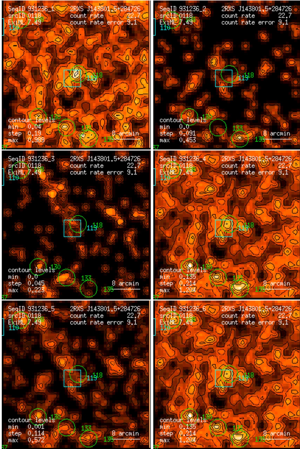
Figure 118: RASS 931236: detection 0118: band rate images, Gaussian filter: (1) PSPC channels 11 – 41, (2) 52 – 90, (3) 91 – 201, (4) 11 – 235, (5) 52 – 201, (6) 11 – 201. Broad band rates in counts/ks. Band rate contour levels in counts/ks/arcmin 2 .
