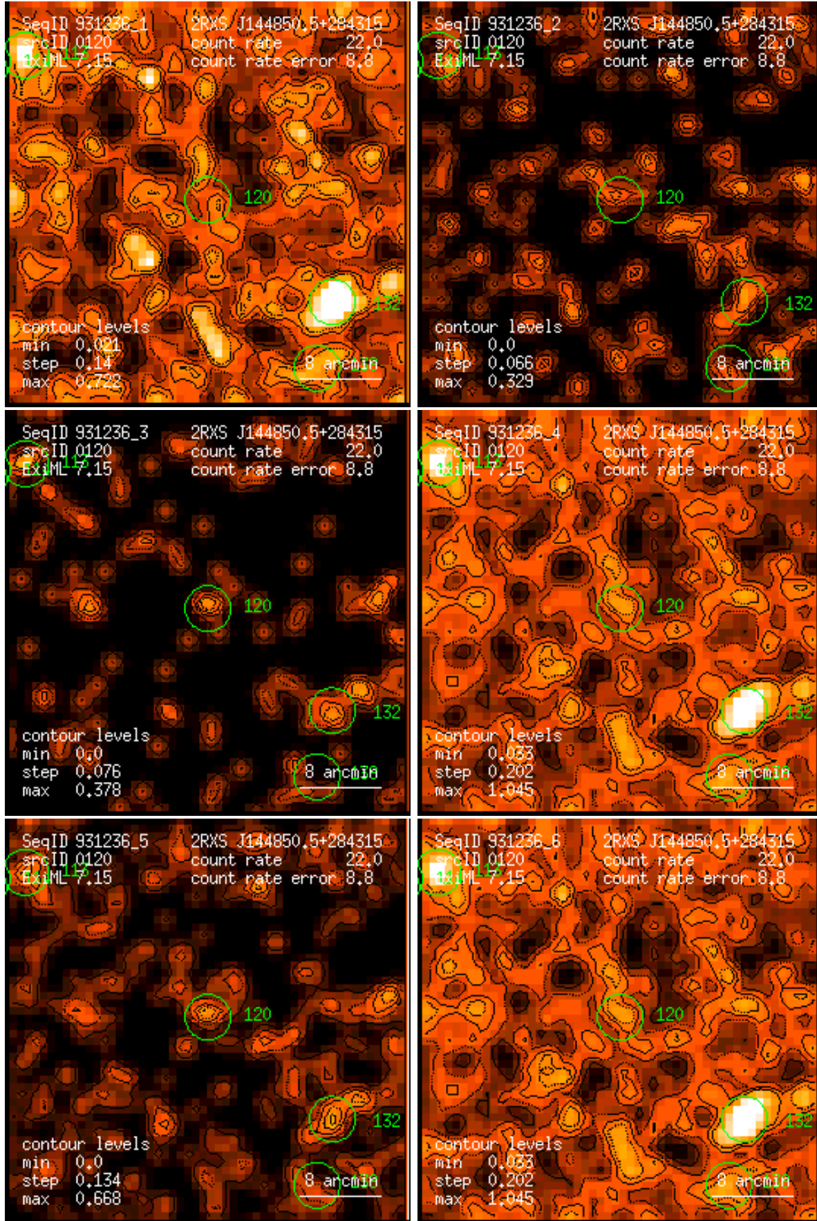
Figure 120: RASS 931236: detection 0120: band rate images, Gaussian filter: (1) PSPC channels 11 – 41, (2) 52 – 90, (3) 91 – 201, (4) 11 – 235, (5) 52 – 201, (6) 11 – 201. Broad band rates in counts/ks. Band rate contour levels in counts/ks/arcmin 2 .
