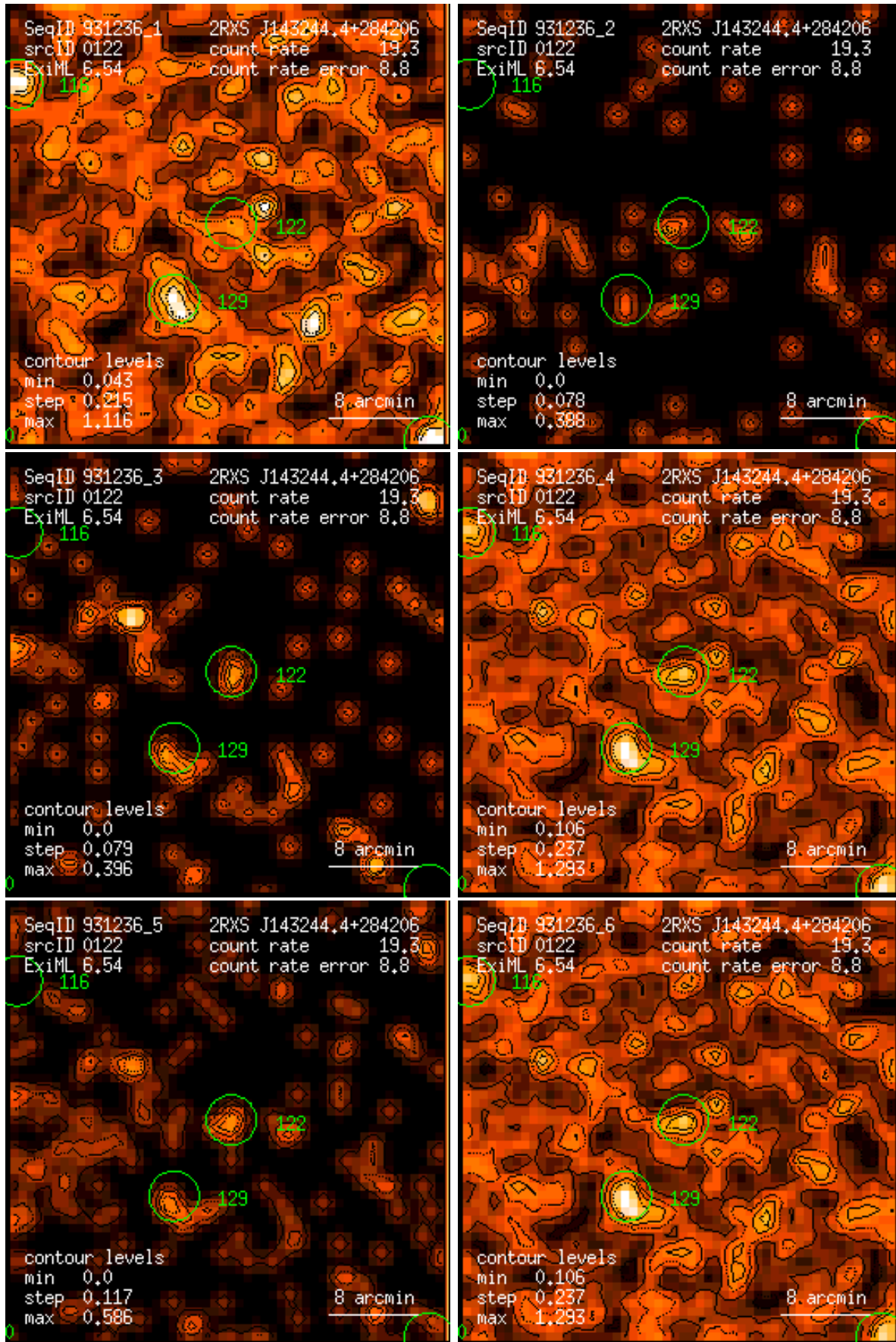
Figure 122: RASS 931236: detection 0122: band rate images, Gaussian filter: (1) PSPC channels 11 – 41, (2) 52 – 90, (3) 91 – 201, (4) 11 – 235, (5) 52 – 201, (6) 11 – 201. Broad band rates in counts/ks. Band rate contour levels in counts/ks/arcmin 2 .
