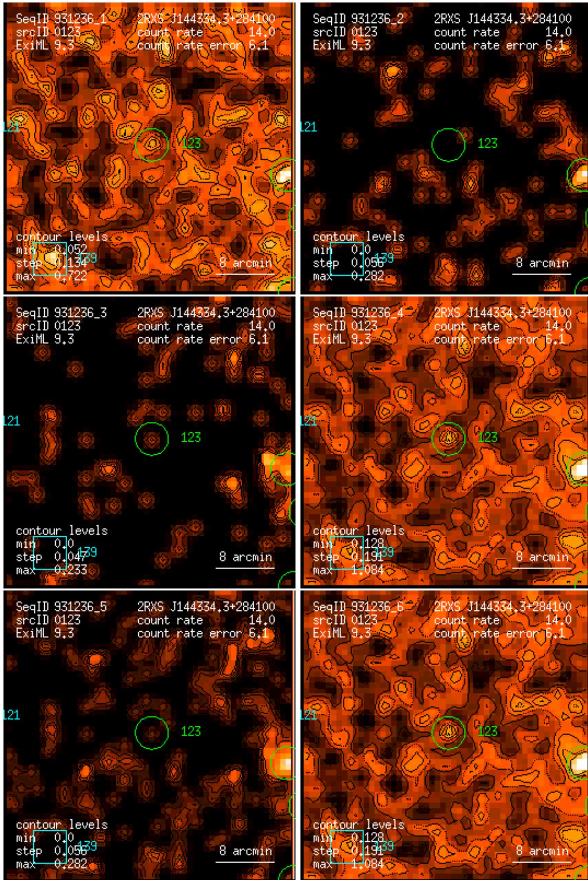
Figure 123: RASS 931236: detection 0123: band rate images, Gaussian filter: (1) PSPC channels 11 – 41, (2) 52 – 90, (3) 91 – 201, (4) 11 – 235, (5) 52 – 201, (6) 11 – 201. Broad band rates in counts/ks. Band rate contour levels in counts/ks/arcmin 2 .
