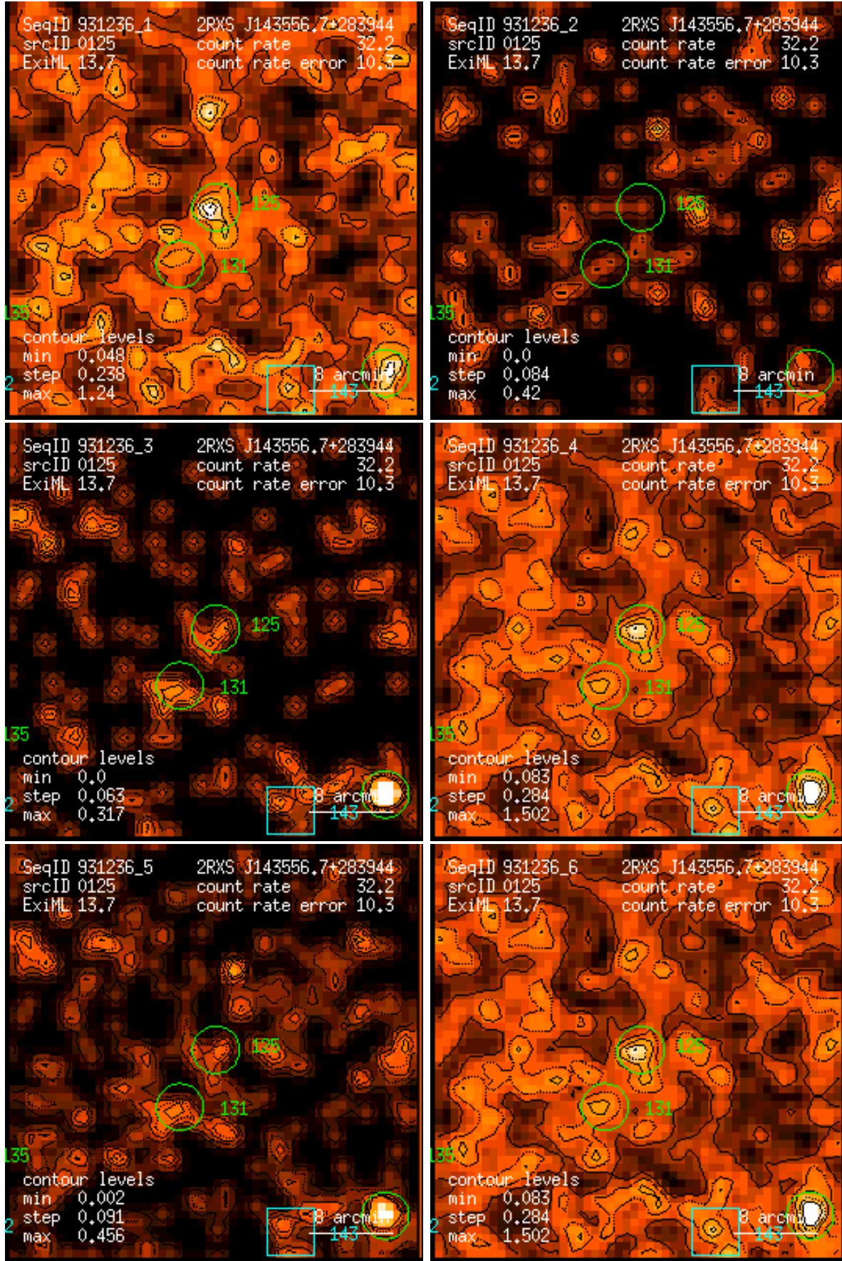
Figure 125: RASS 931236: detection 0125: band rate images, Gaussian filter: (1) PSPC channels 11 – 41, (2) 52 – 90, (3) 91 – 201, (4) 11 – 235, (5) 52 – 201, (6) 11 – 201. Broad band rates in counts/ks. Band rate contour levels in counts/ks/arcmin 2 .
