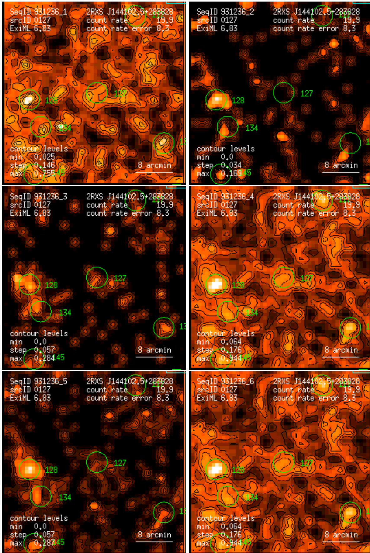
Figure 127: RASS 931236: detection 0127: band rate images, Gaussian filter: (1) PSPC channels 11 – 41, (2) 52 – 90, (3) 91 – 201, (4) 11 – 235, (5) 52 – 201, (6) 11 – 201. Broad band rates in counts/ks. Band rate contour levels in counts/ks/arcmin 2 .
