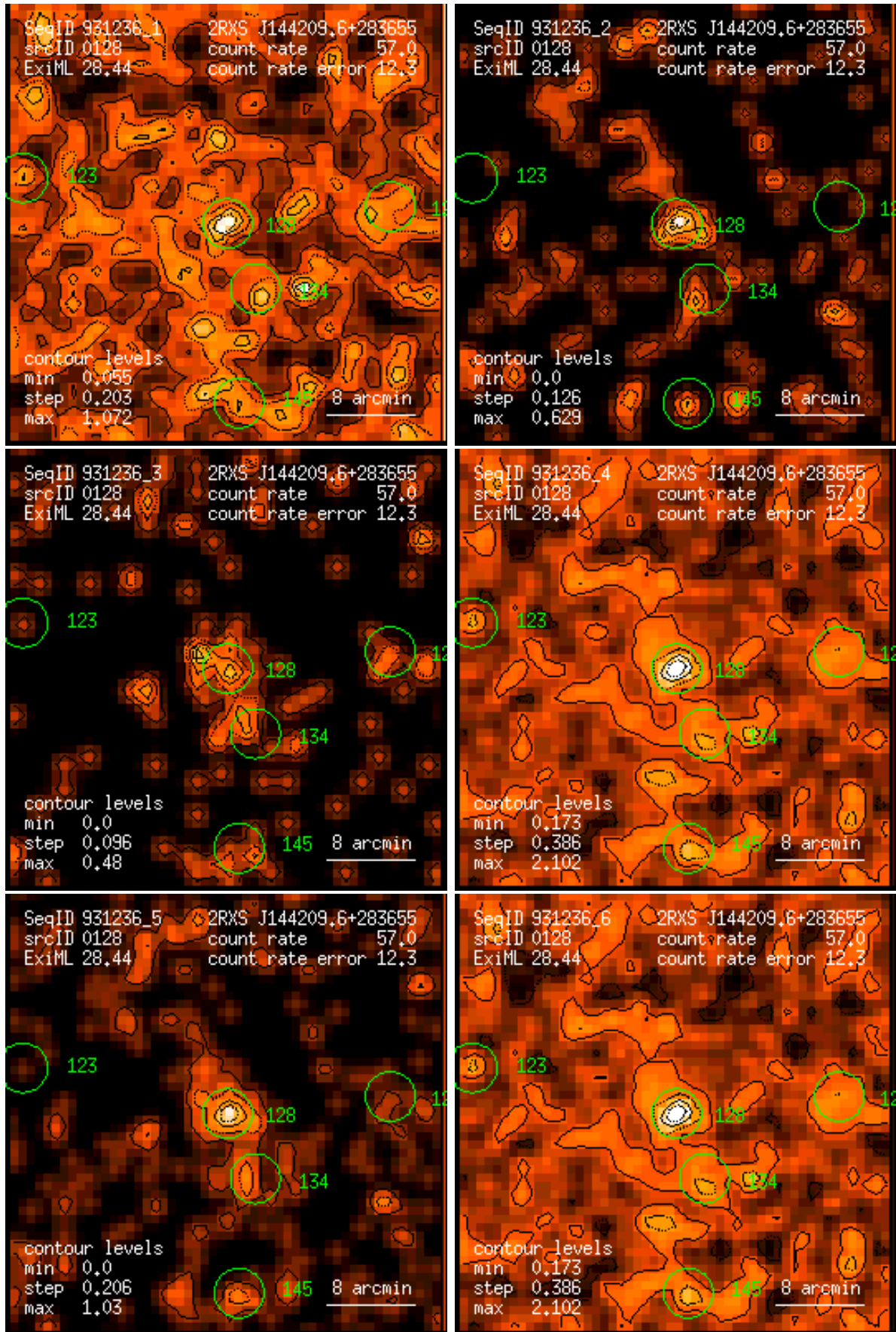
Figure 128: RASS 931236: detection 0128: band rate images, Gaussian filter: (1) PSPC channels 11 – 41, (2) 52 – 90, (3) 91 – 201, (4) 11 – 235, (5) 52 – 201, (6) 11 – 201. Broad band rates in counts/ks. Band rate contour levels in counts/ks/arcmin 2 .
