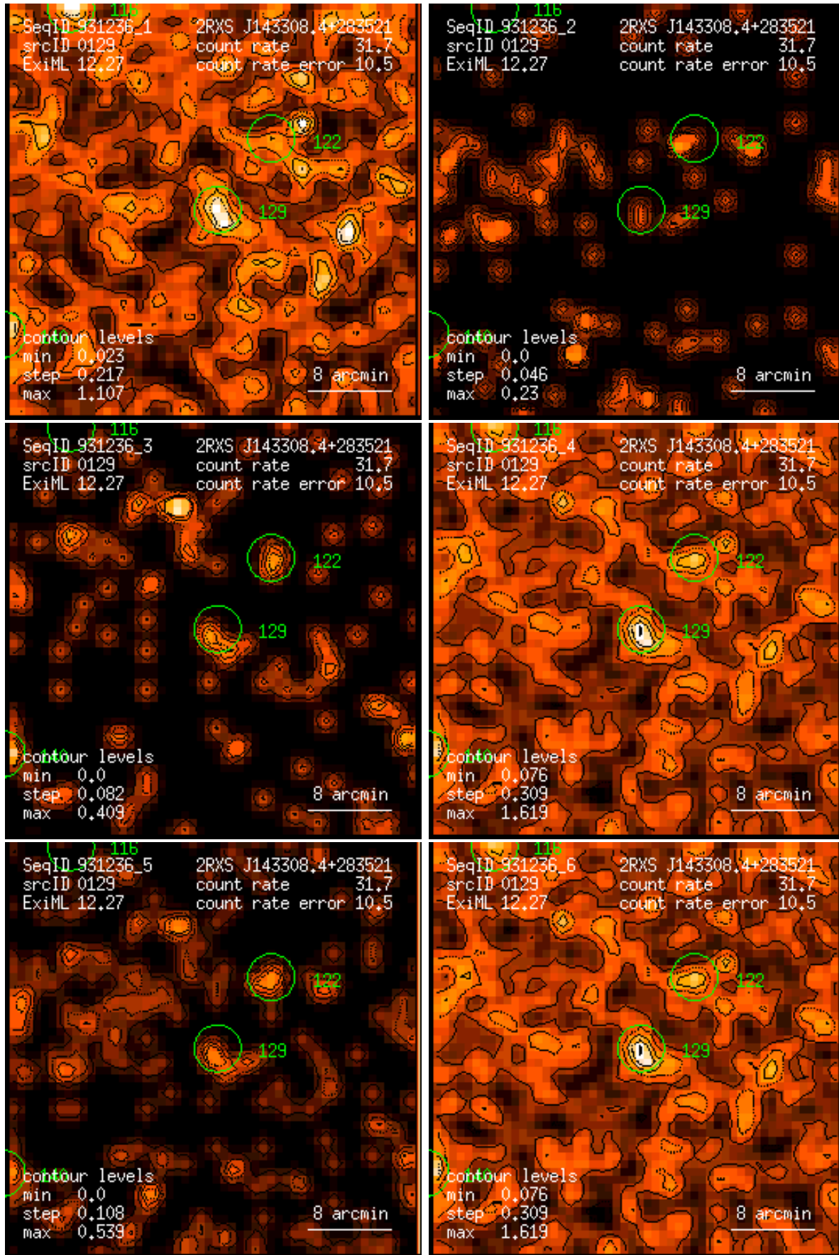
Figure 129: RASS 931236: detection 0129: band rate images, Gaussian filter: (1) PSPC channels 11 – 41, (2) 52 – 90, (3) 91 – 201, (4) 11 – 235, (5) 52 – 201, (6) 11 – 201. Broad band rates in counts/ks. Band rate contour levels in counts/ks/arcmin 2 .
