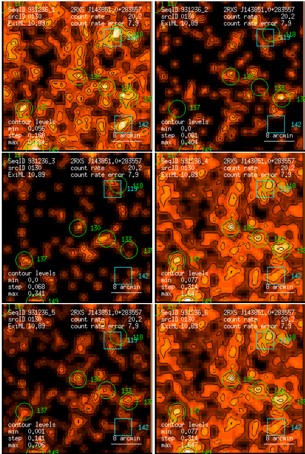
Figure 130: RASS 931236: detection 0130: band rate images, Gaussian filter: (1) PSPC channels 11 – 41, (2) 52 – 90, (3) 91 – 201, (4) 11 – 235, (5) 52 – 201, (6) 11 – 201. Broad band rates in counts/ks. Band rate contour levels in counts/ks/arcmin 2 .
