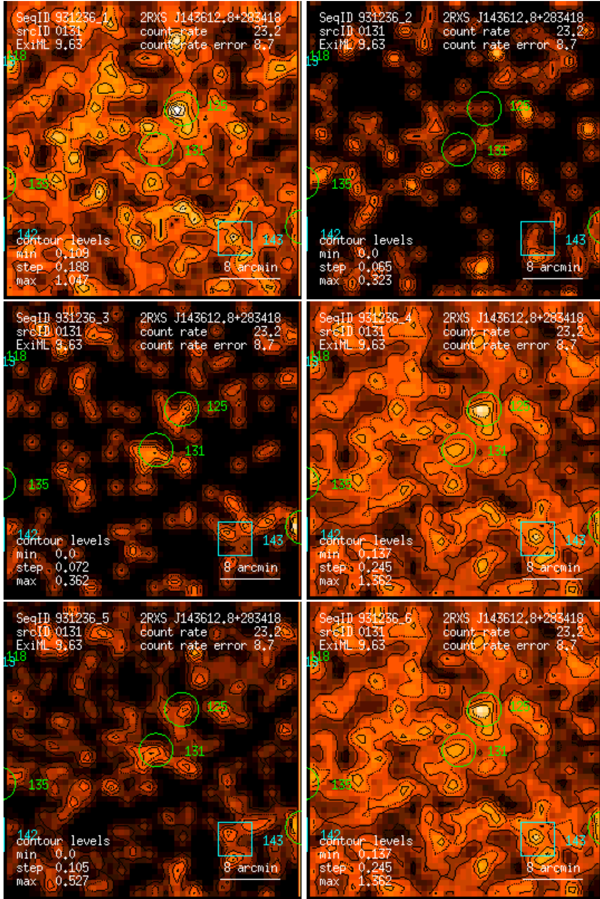
Figure 131: RASS 931236: detection 0131: band rate images, Gaussian filter: (1) PSPC channels 11 – 41, (2) 52 – 90, (3) 91 – 201, (4) 11 – 235, (5) 52 – 201, (6) 11 – 201. Broad band rates in counts/ks. Band rate contour levels in counts/ks/arcmin 2 .
