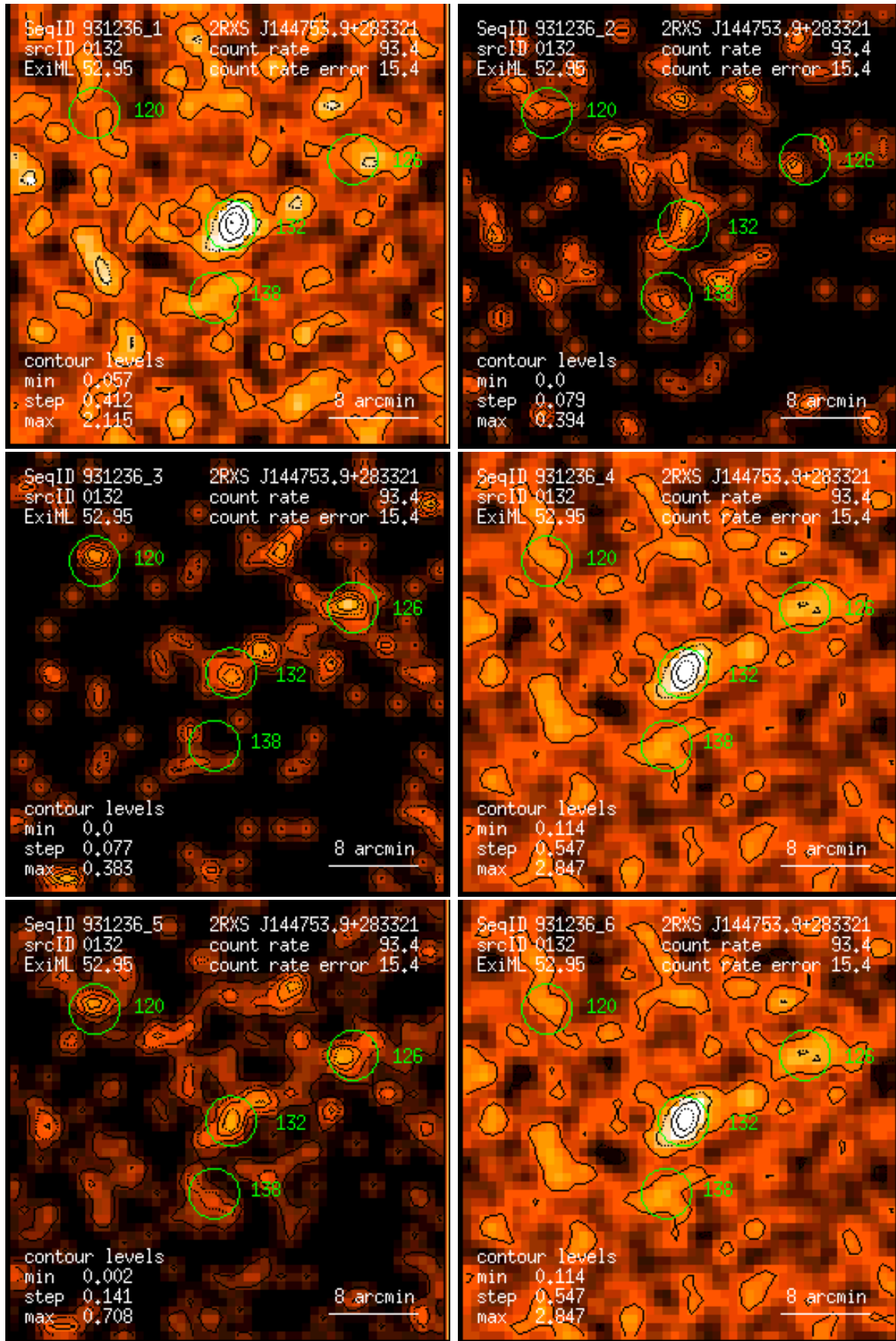
Figure 132: RASS 931236: detection 0132: band rate images, Gaussian filter: (1) PSPC channels 11 – 41, (2) 52 – 90, (3) 91 – 201, (4) 11 – 235, (5) 52 – 201, (6) 11 – 201. Broad band rates in counts/ks. Band rate contour levels in counts/ks/arcmin 2 .
