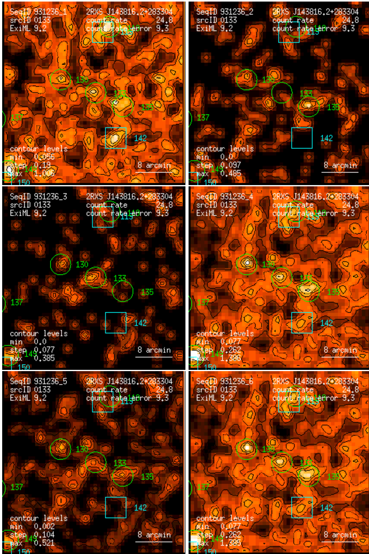
Figure 133: RASS 931236: detection 0133: band rate images, Gaussian filter: (1) PSPC channels 11 – 41, (2) 52 – 90, (3) 91 – 201, (4) 11 – 235, (5) 52 – 201, (6) 11 – 201. Broad band rates in counts/ks. Band rate contour levels in counts/ks/arcmin 2 .
