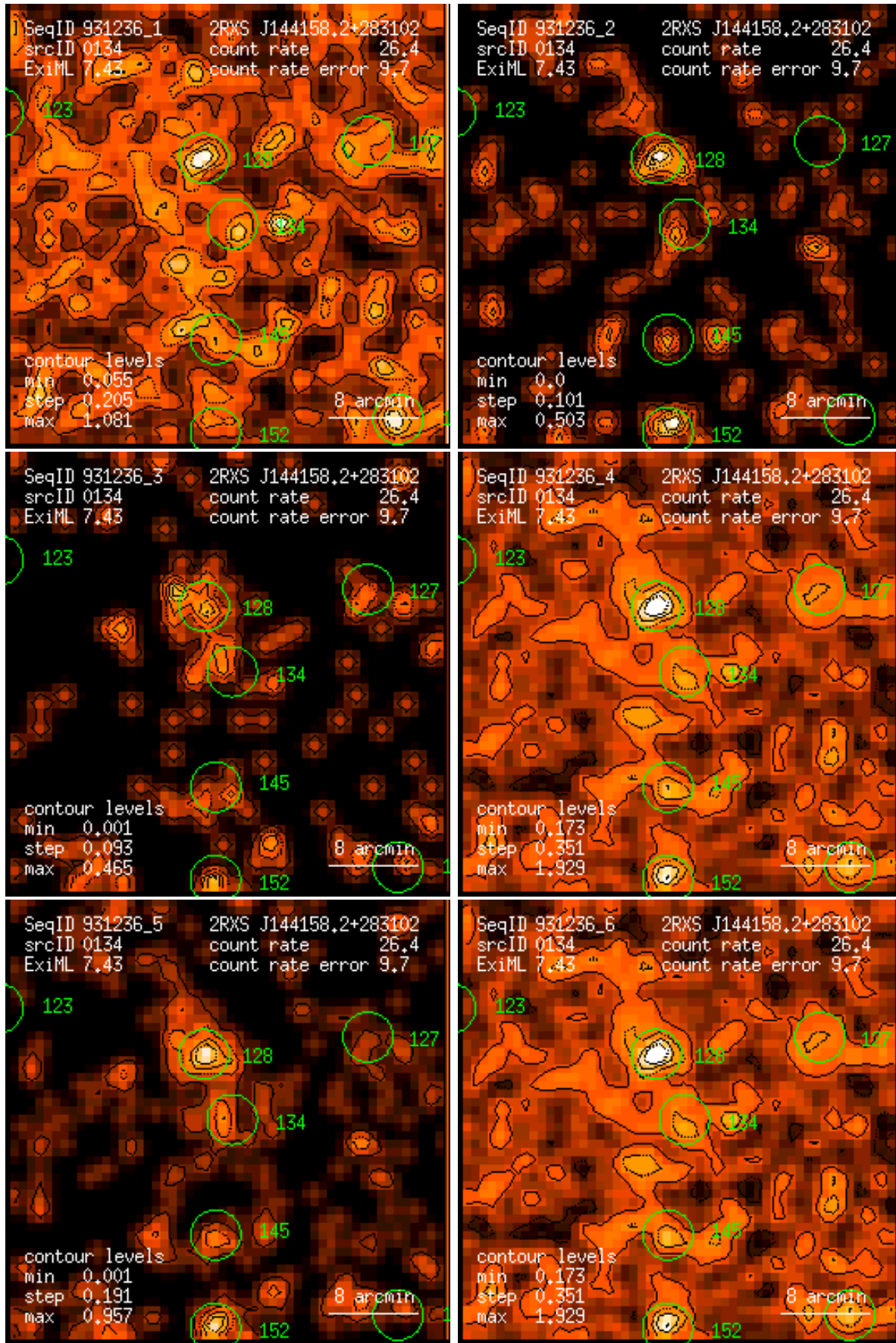
Figure 134: RASS 931236: detection 0134: band rate images, Gaussian filter: (1) PSPC channels 11 – 41, (2) 52 – 90, (3) 91 – 201, (4) 11 – 235, (5) 52 – 201, (6) 11 – 201. Broad band rates in counts/ks. Band rate contour levels in counts/ks/arcmin 2 .
