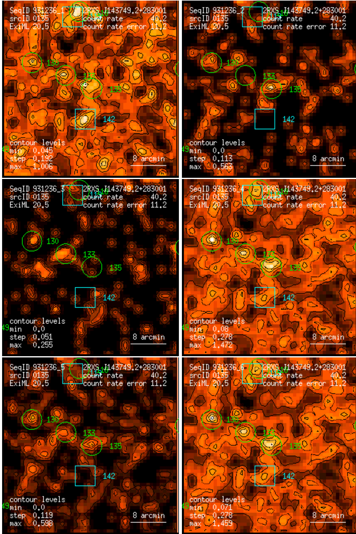
Figure 135: RASS 931236: detection 0135: band rate images, Gaussian filter: (1) PSPC channels 11 – 41, (2) 52 – 90, (3) 91 – 201, (4) 11 – 235, (5) 52 – 201, (6) 11 – 201. Broad band rates in counts/ks. Band rate contour levels in counts/ks/arcmin 2 .
