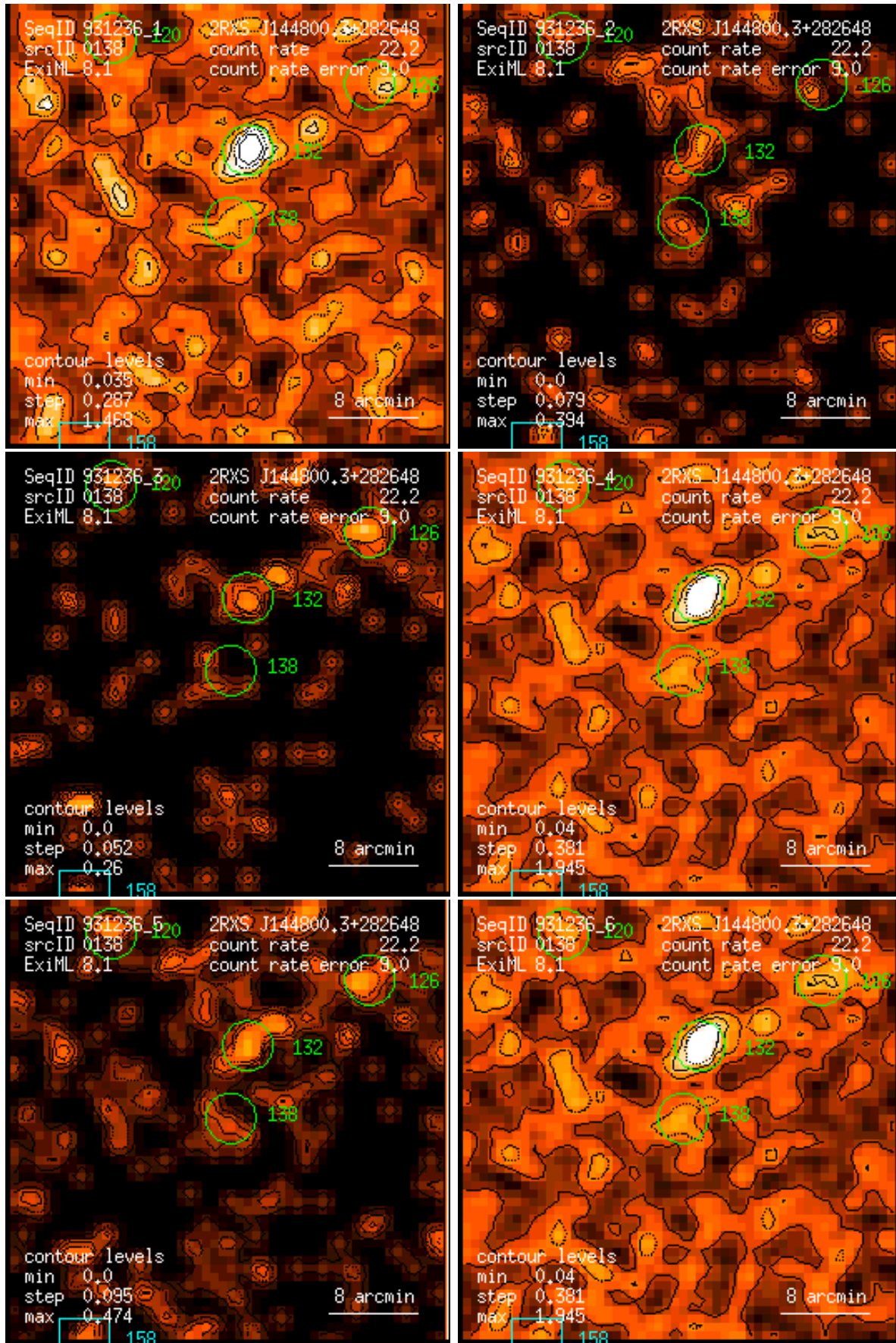
Figure 138: RASS 931236: detection 0138: band rate images, Gaussian filter: (1) PSPC channels 11 – 41, (2) 52 – 90, (3) 91 – 201, (4) 11 – 235, (5) 52 – 201, (6) 11 – 201. Broad band rates in counts/ks. Band rate contour levels in counts/ks/arcmin 2 .
