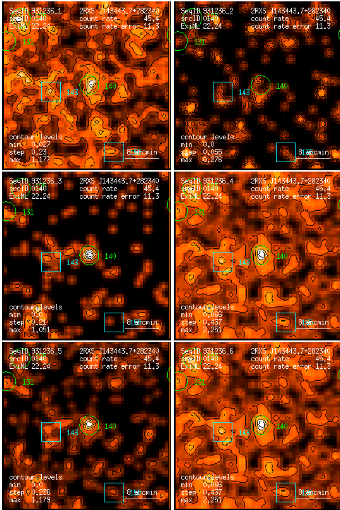
Figure 140: RASS 931236: detection 0140: band rate images, Gaussian filter: (1) PSPC channels 11 – 41, (2) 52 – 90, (3) 91 – 201, (4) 11 – 235, (5) 52 – 201, (6) 11 – 201. Broad band rates in counts/ks. Band rate contour levels in counts/ks/arcmin 2 .
