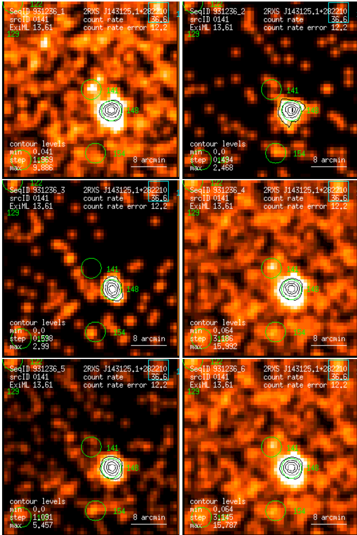
Figure 141: RASS 931236: detection 0141: band rate images, Gaussian filter: (1) PSPC channels 11 – 41, (2) 52 – 90, (3) 91 – 201, (4) 11 – 235, (5) 52 – 201, (6) 11 – 201. Broad band rates in counts/ks. Band rate contour levels in counts/ks/arcmin 2 .
