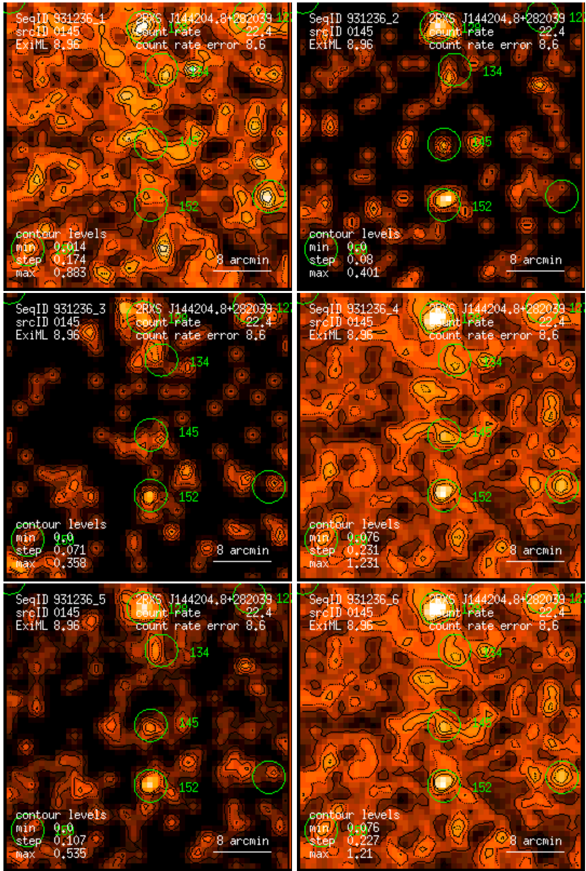
Figure 145: RASS 931236: detection 0145: band rate images, Gaussian filter: (1) PSPC channels 11 – 41, (2) 52 – 90, (3) 91 – 201, (4) 11 – 235, (5) 52 – 201, (6) 11 – 201. Broad band rates in counts/ks. Band rate contour levels in counts/ks/arcmin 2 .
