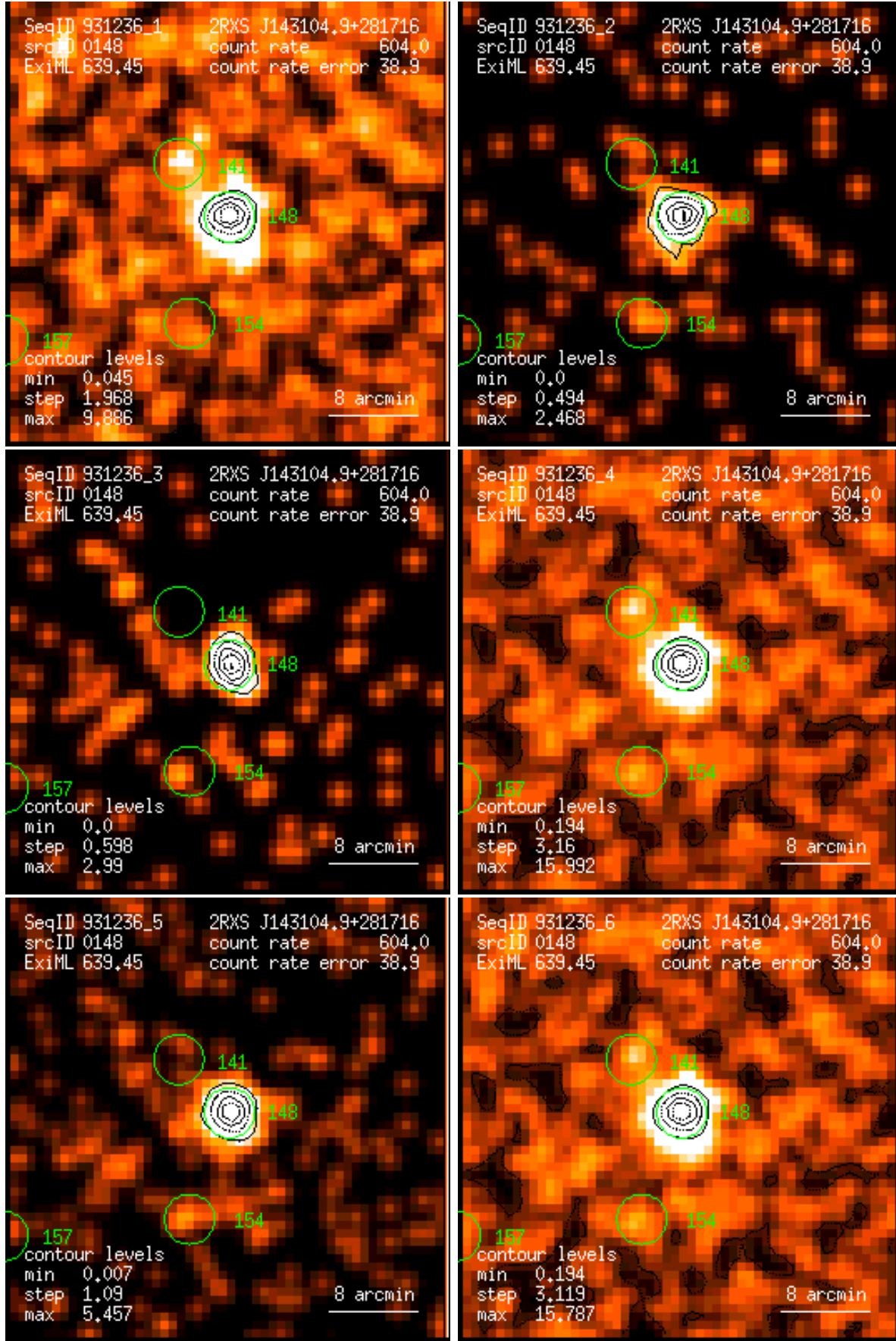
Figure 148: RASS 931236: detection 0148: band rate images, Gaussian filter: (1) PSPC channels 11 – 41, (2) 52 – 90, (3) 91 – 201, (4) 11 – 235, (5) 52 – 201, (6) 11 – 201. Broad band rates in counts/ks. Band rate contour levels in counts/ks/arcmin 2 .
