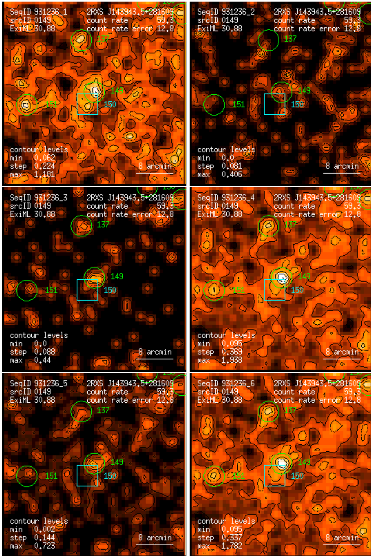
Figure 149: RASS 931236: detection 0149: band rate images, Gaussian filter: (1) PSPC channels 11 – 41, (2) 52 – 90, (3) 91 – 201, (4) 11 – 235, (5) 52 – 201, (6) 11 – 201. Broad band rates in counts/ks. Band rate contour levels in counts/ks/arcmin 2 .
