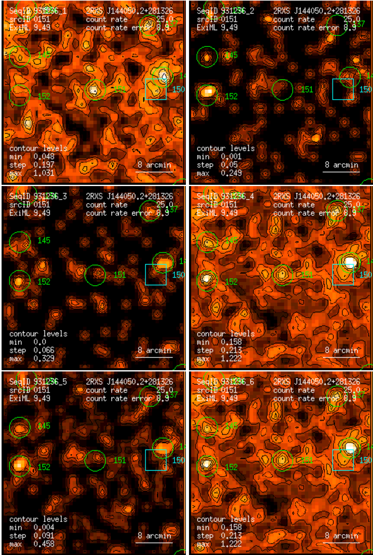
Figure 151: RASS 931236: detection 0151: band rate images, Gaussian filter: (1) PSPC channels 11 – 41, (2) 52 – 90, (3) 91 – 201, (4) 11 – 235, (5) 52 – 201, (6) 11 – 201. Broad band rates in counts/ks. Band rate contour levels in counts/ks/arcmin 2 .
