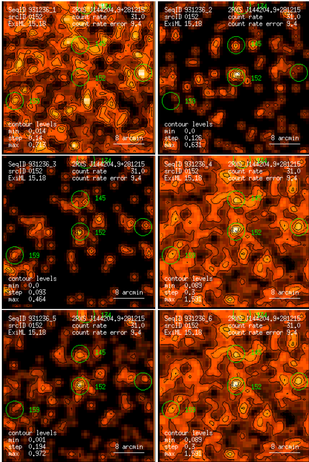
Figure 152: RASS 931236: detection 0152: band rate images, Gaussian filter: (1) PSPC channels 11 – 41, (2) 52 – 90, (3) 91 – 201, (4) 11 – 235, (5) 52 – 201, (6) 11 – 201. Broad band rates in counts/ks. Band rate contour levels in counts/ks/arcmin 2 .
