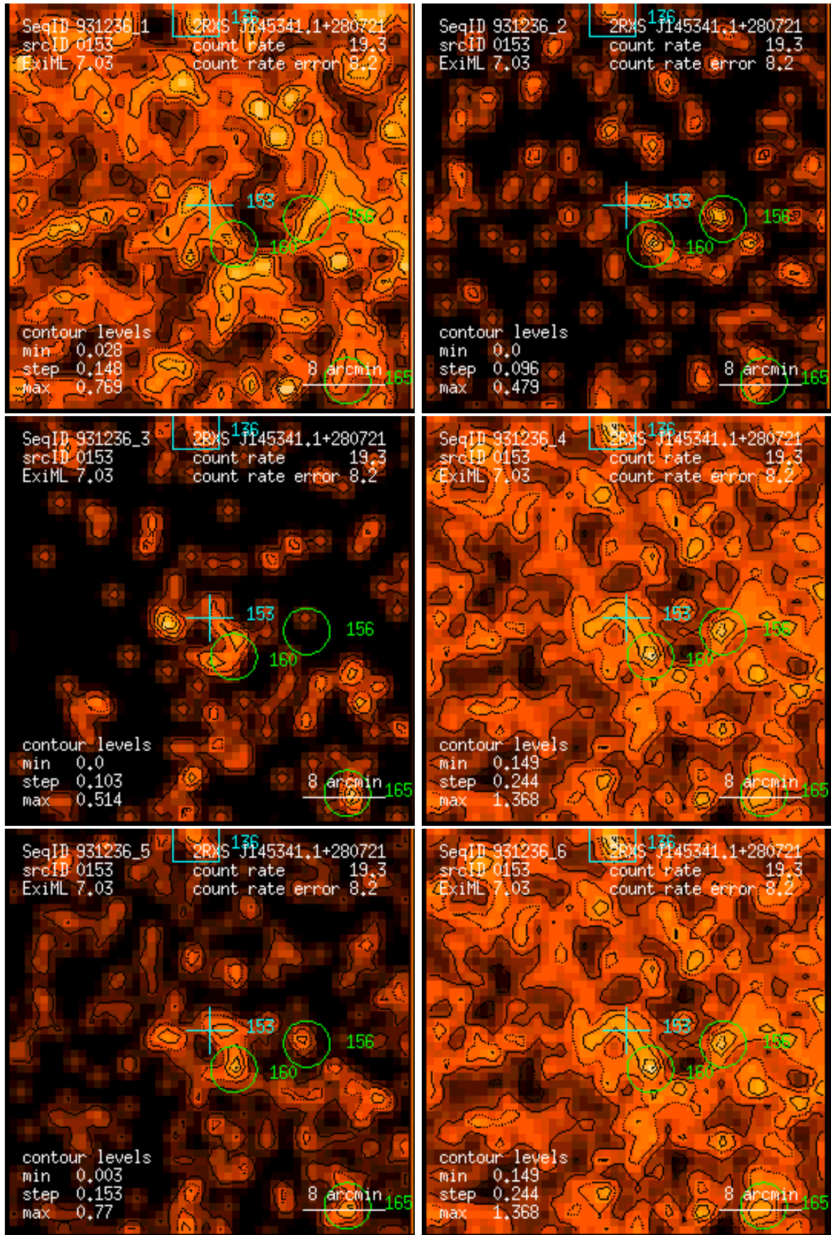
Figure 153: RASS 931236: detection 0153: band rate images, Gaussian filter: (1) PSPC channels 11 – 41, (2) 52 – 90, (3) 91 – 201, (4) 11 – 235, (5) 52 – 201, (6) 11 – 201. Broad band rates in counts/ks. Band rate contour levels in counts/ks/arcmin 2 .
