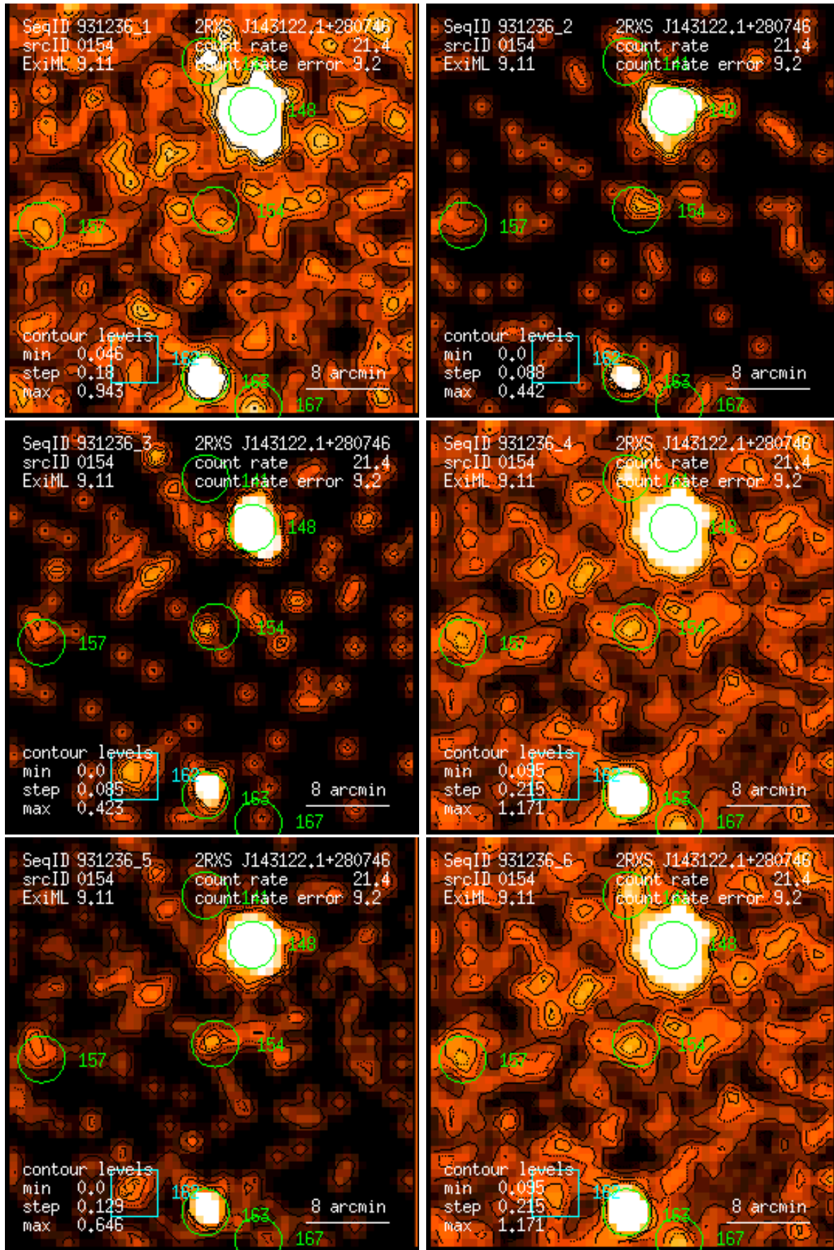
Figure 154: RASS 931236: detection 0154: band rate images, Gaussian filter: (1) PSPC channels 11 – 41, (2) 52 – 90, (3) 91 – 201, (4) 11 – 235, (5) 52 – 201, (6) 11 – 201. Broad band rates in counts/ks. Band rate contour levels in counts/ks/arcmin 2 .
